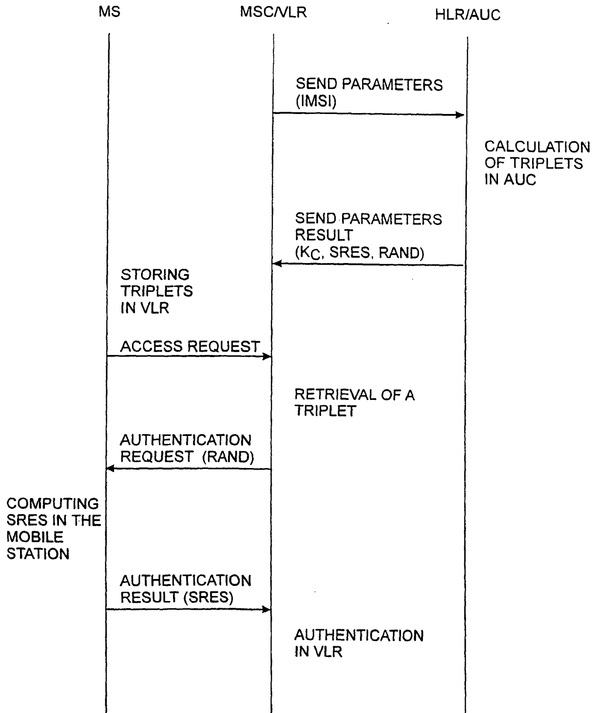
Fig. 5 (PRIOR ART)
