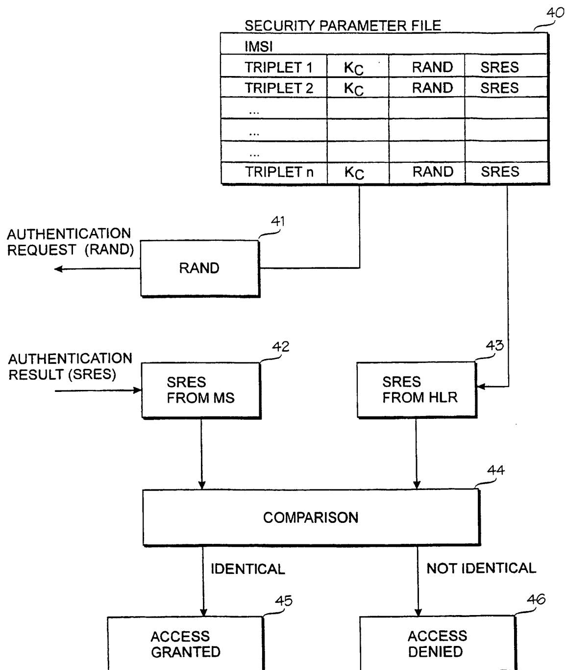
Fig. 4 (PRIOR ART)
