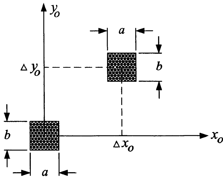
IR Diffracton at a Rectangular Aperture
