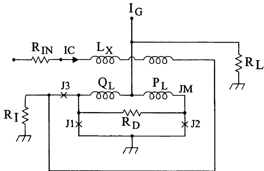
Circuit of Refractory Josephson OR Gate
