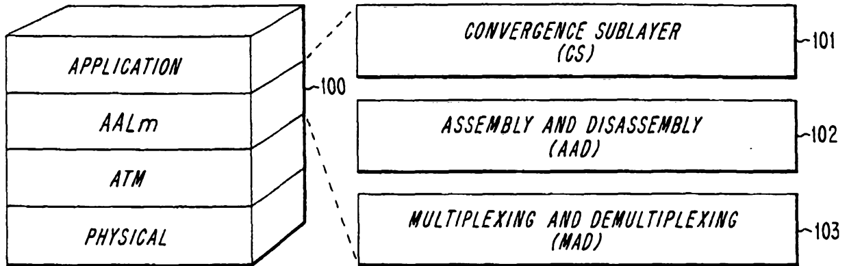
FIG. 1 (PRIOR ART)
