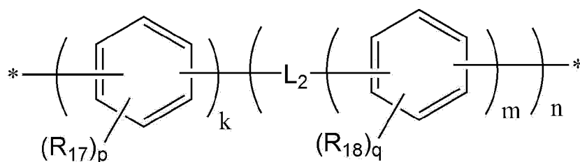
[Chemical Formula 10]
