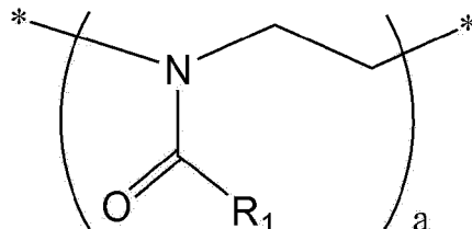
[Chemical Formula 1]
