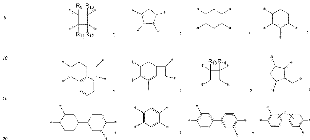
[Chemical Formula 8]
