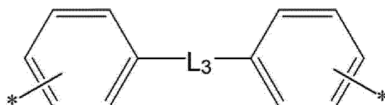
[Chemical Formula 10-2]
