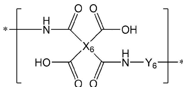
[Chemical Formula 7]
