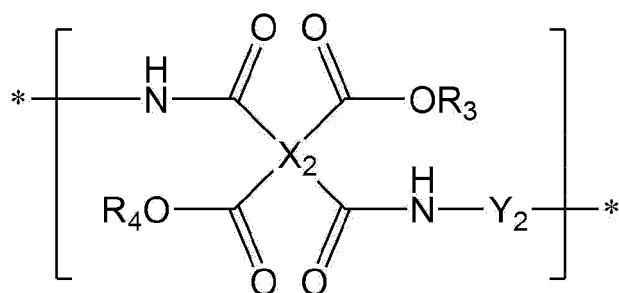
[Chemical Formula 4]
