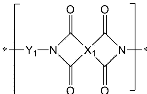
[Chemical Formula 2]
