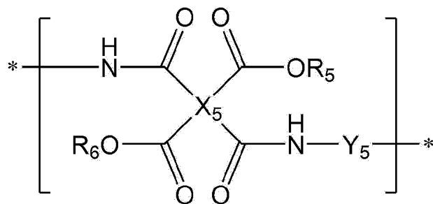
[Chemical Formula 6]
