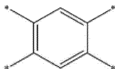
[Chemical Formula 8-2]
