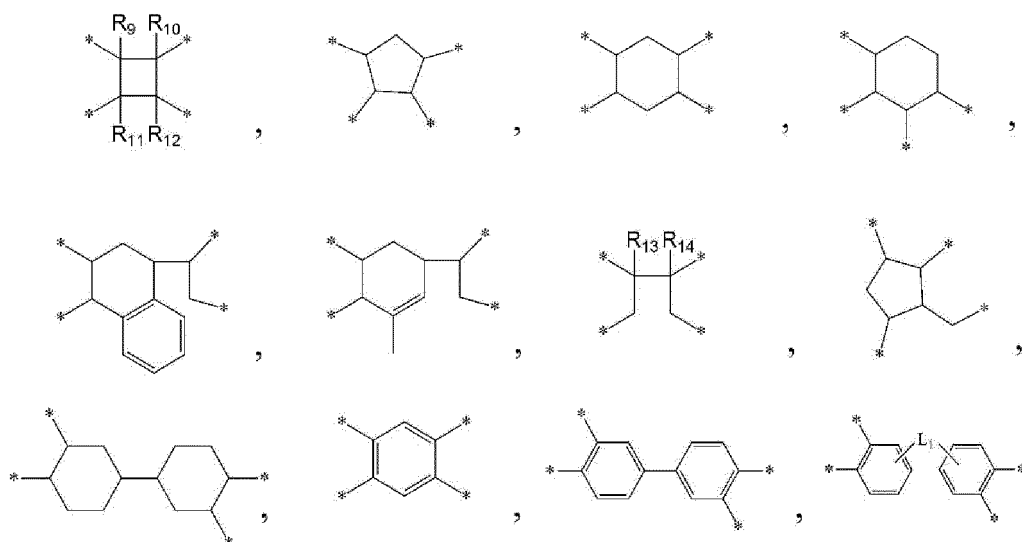
[Chemical Formula 8]
