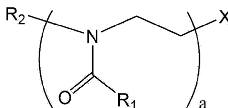
[Chemical Formula 1-1]
