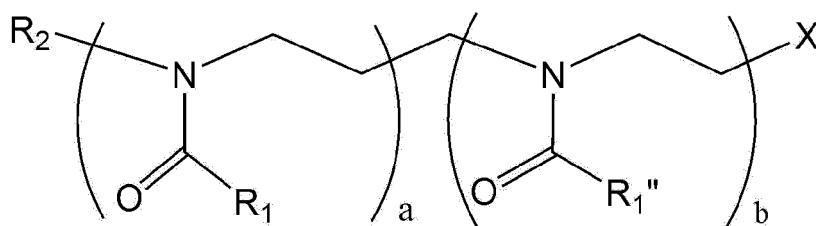
[Chemical Formula 1-2]
