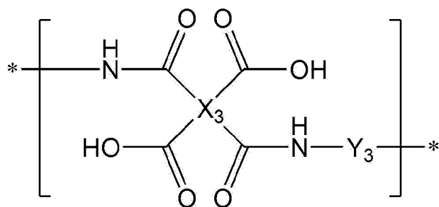
[Chemical Formula 5]
