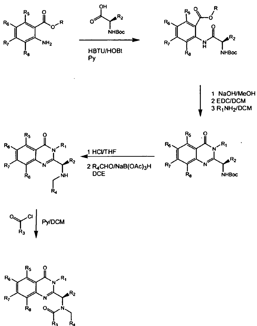
Figure 4: Asymmetric Synthesis
