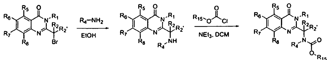
Figure 5c: Urea Synthesis
