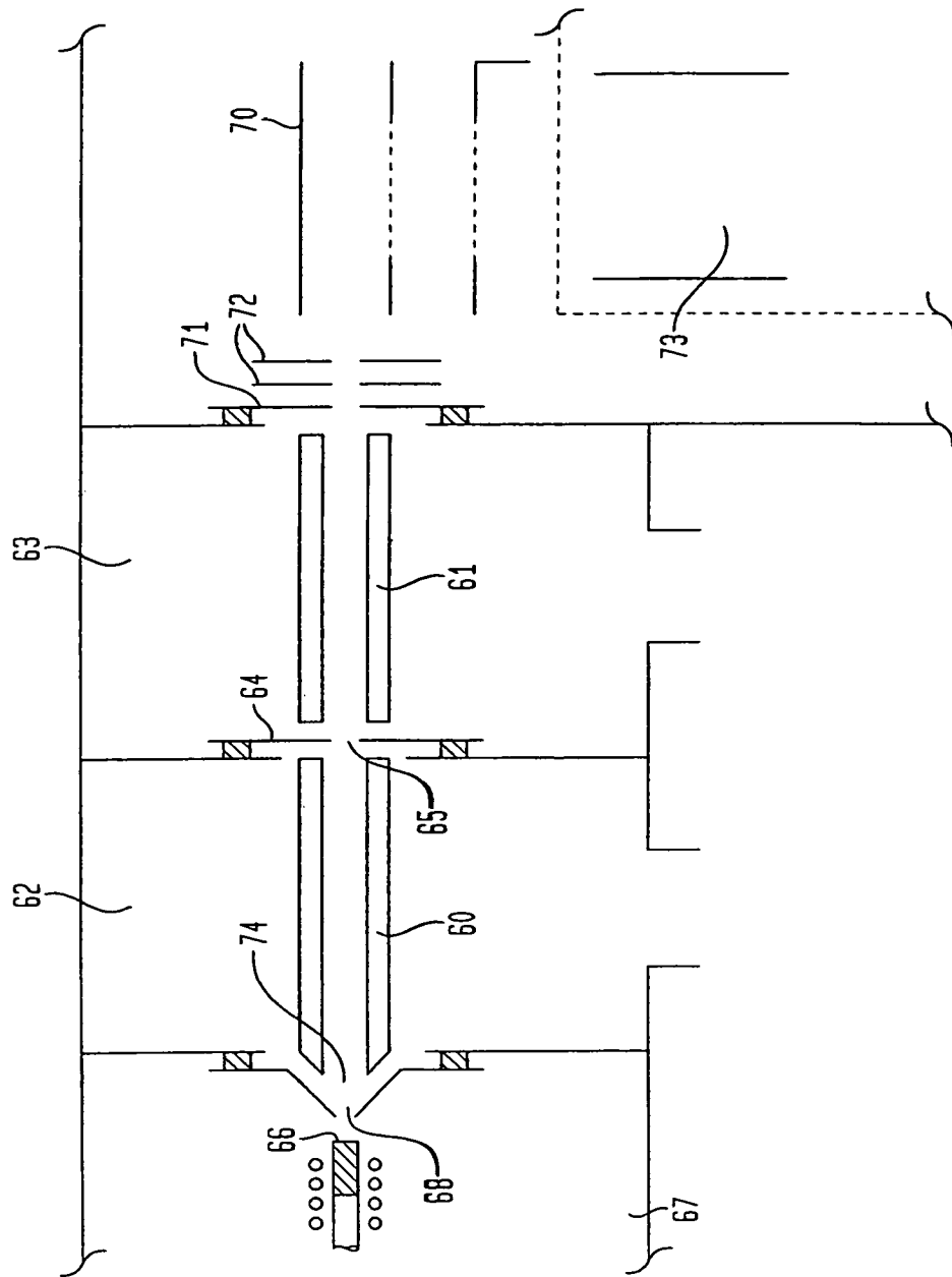
FIG. 3 (PRIOR ART)
