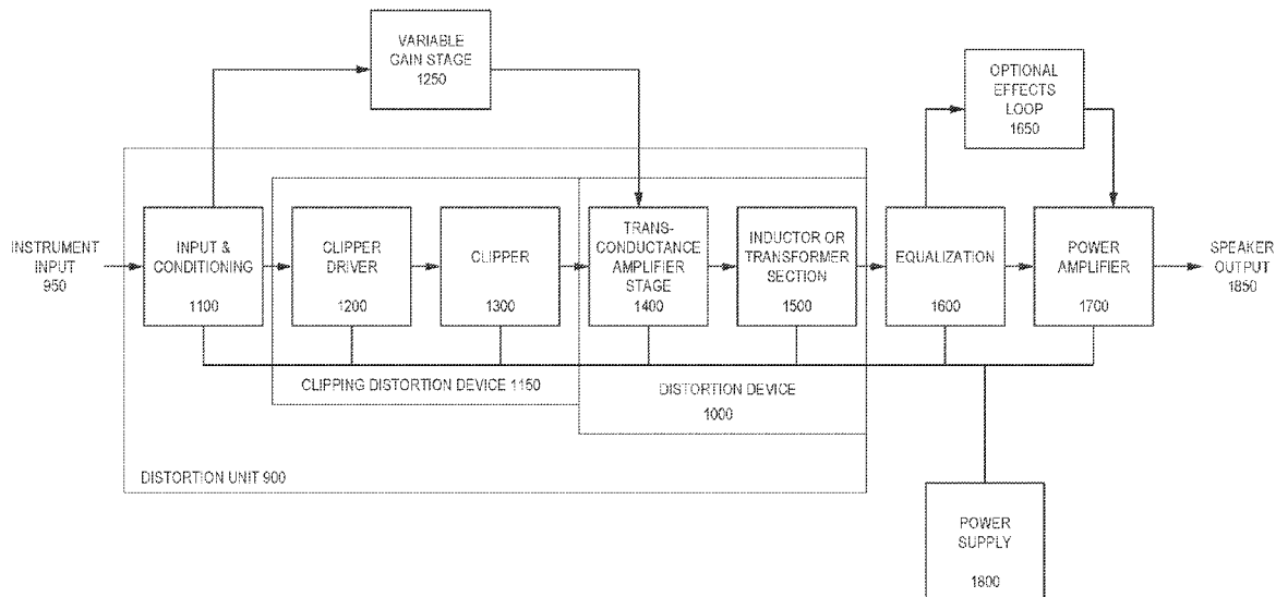
MUSICAL INSTRUMENT AMPLIFIER 800
