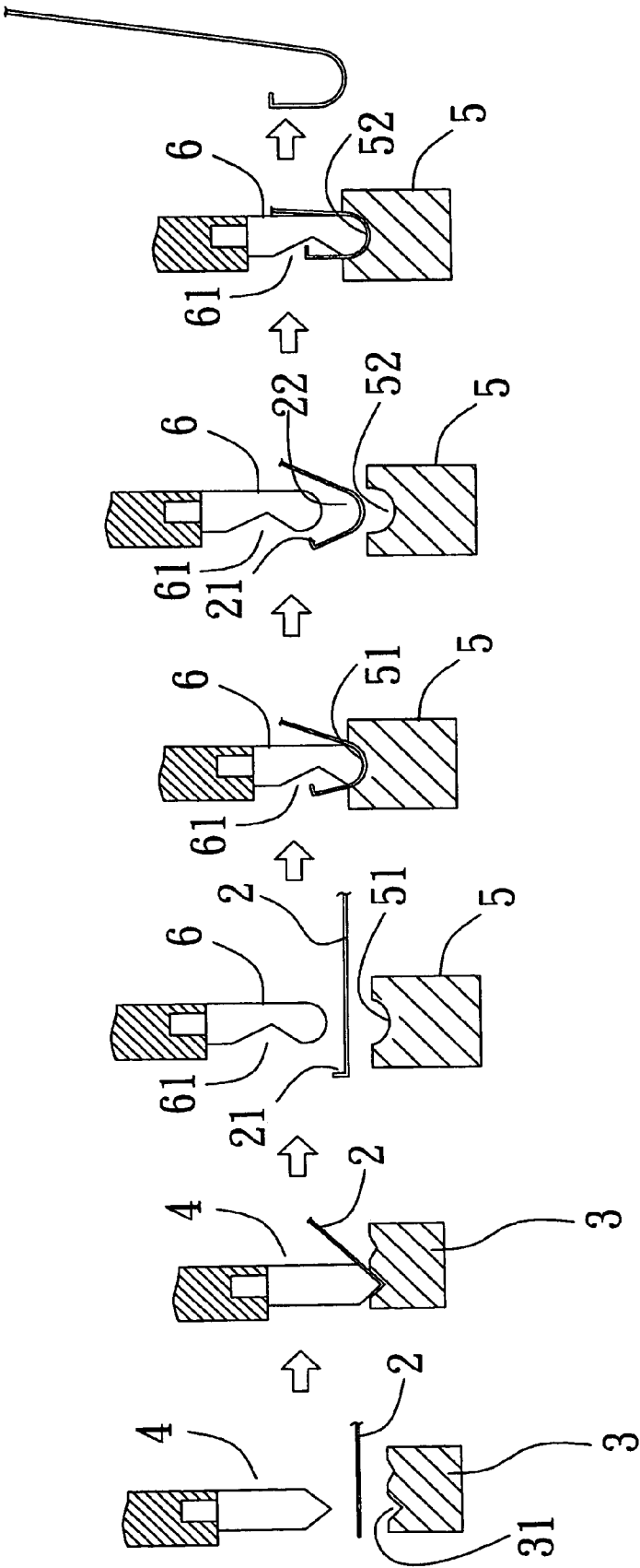
FIG. 4 (PRIOR ART)
