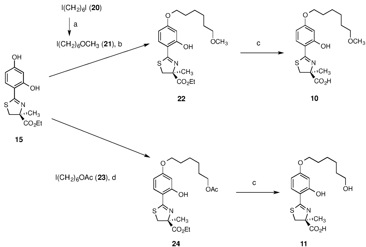
Scheme 2. Synthesis of (S)-4,5-dihydro-2-[2-hydroxy-4-(6-methoxyhexyloxy)phenyl]-4-methyl-4-thiazolecarboxylic acid ( 10 ) and (S)-4,5-dihydro-2-[2-hydroxy-4-(6-hydroxyhexyloxy)phenyl]-4-methyl-4-thiazolecarboxylic acid ( 11 ) a
