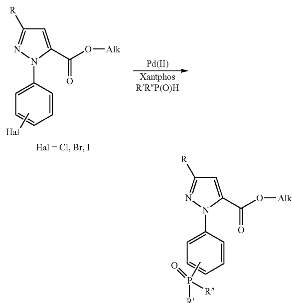
Scheme 16
