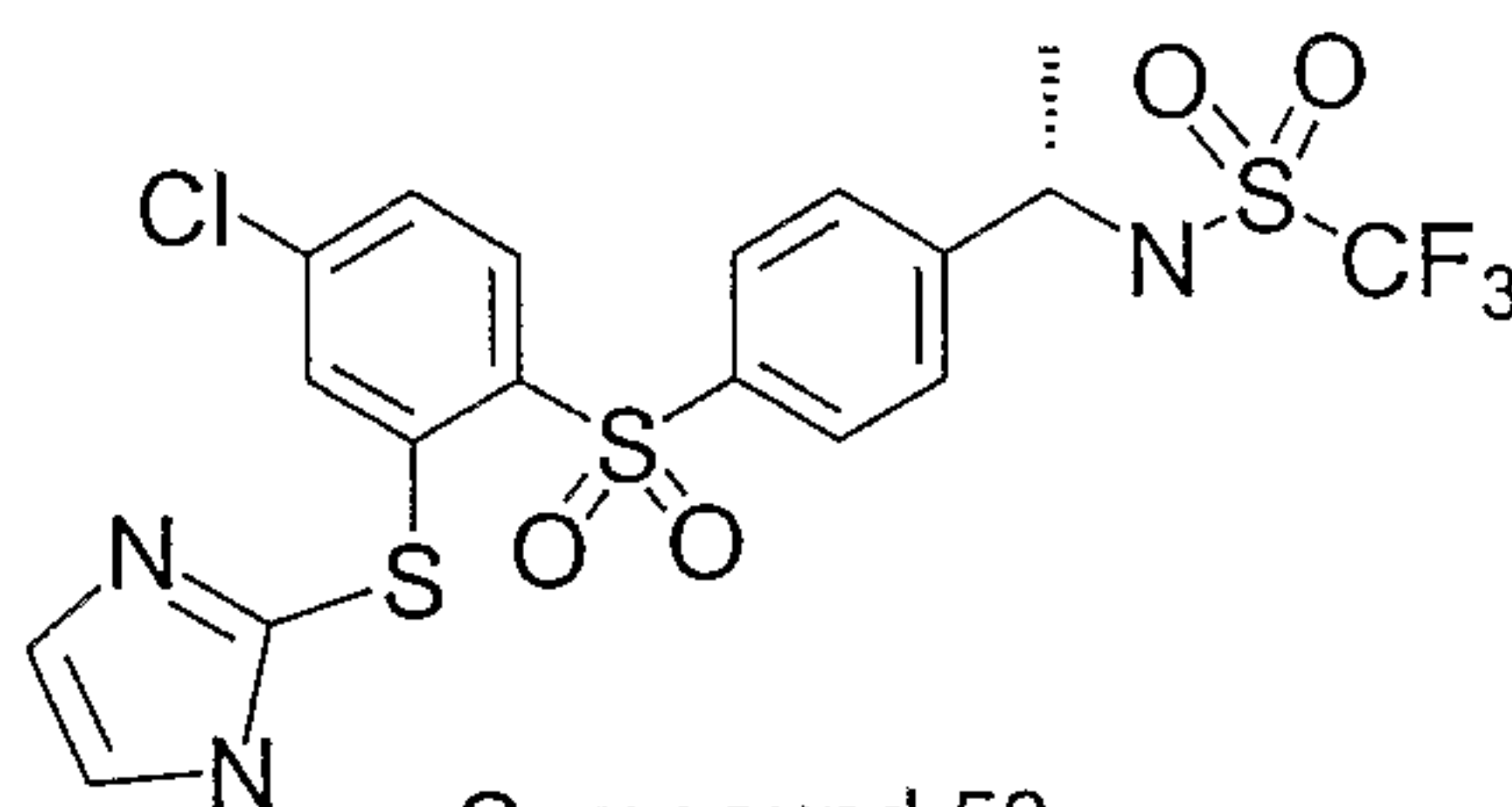
Compound 58
