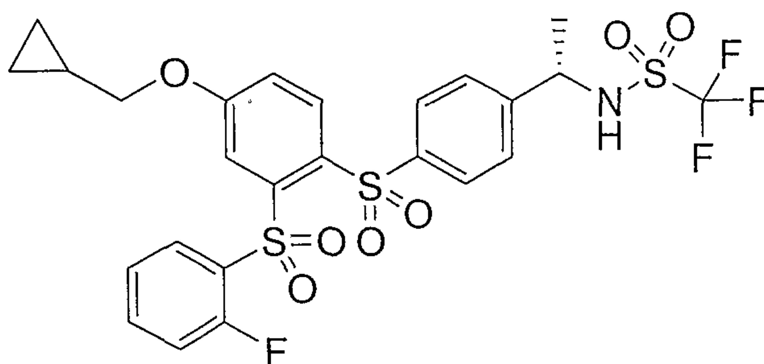
Compound XXXXIII
