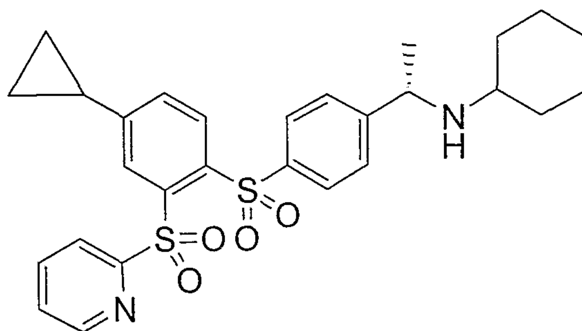
Compound XXXXVIII
