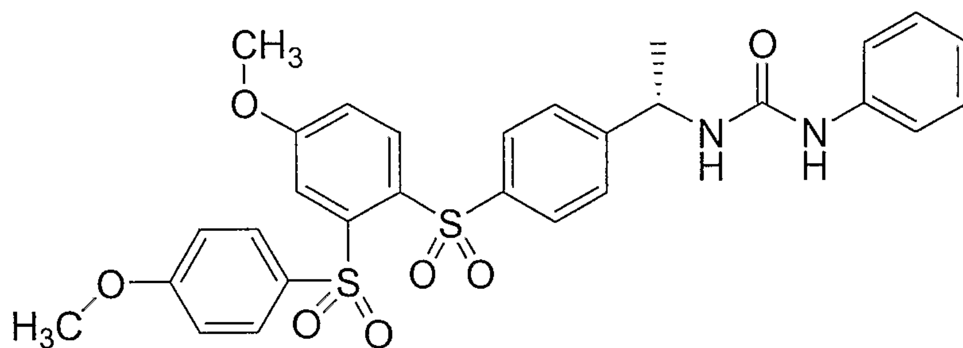
Compound III
