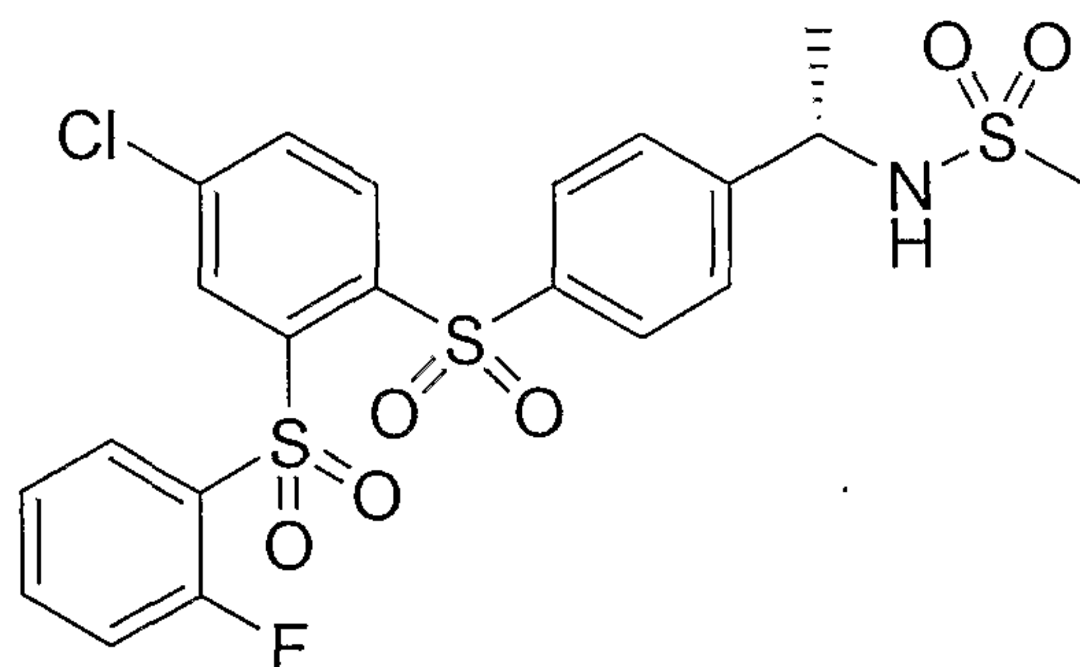
Compound IV
