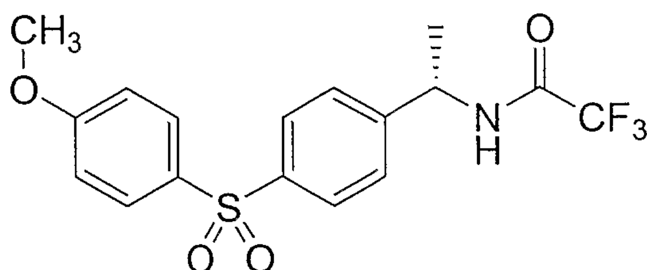
Compound 2
