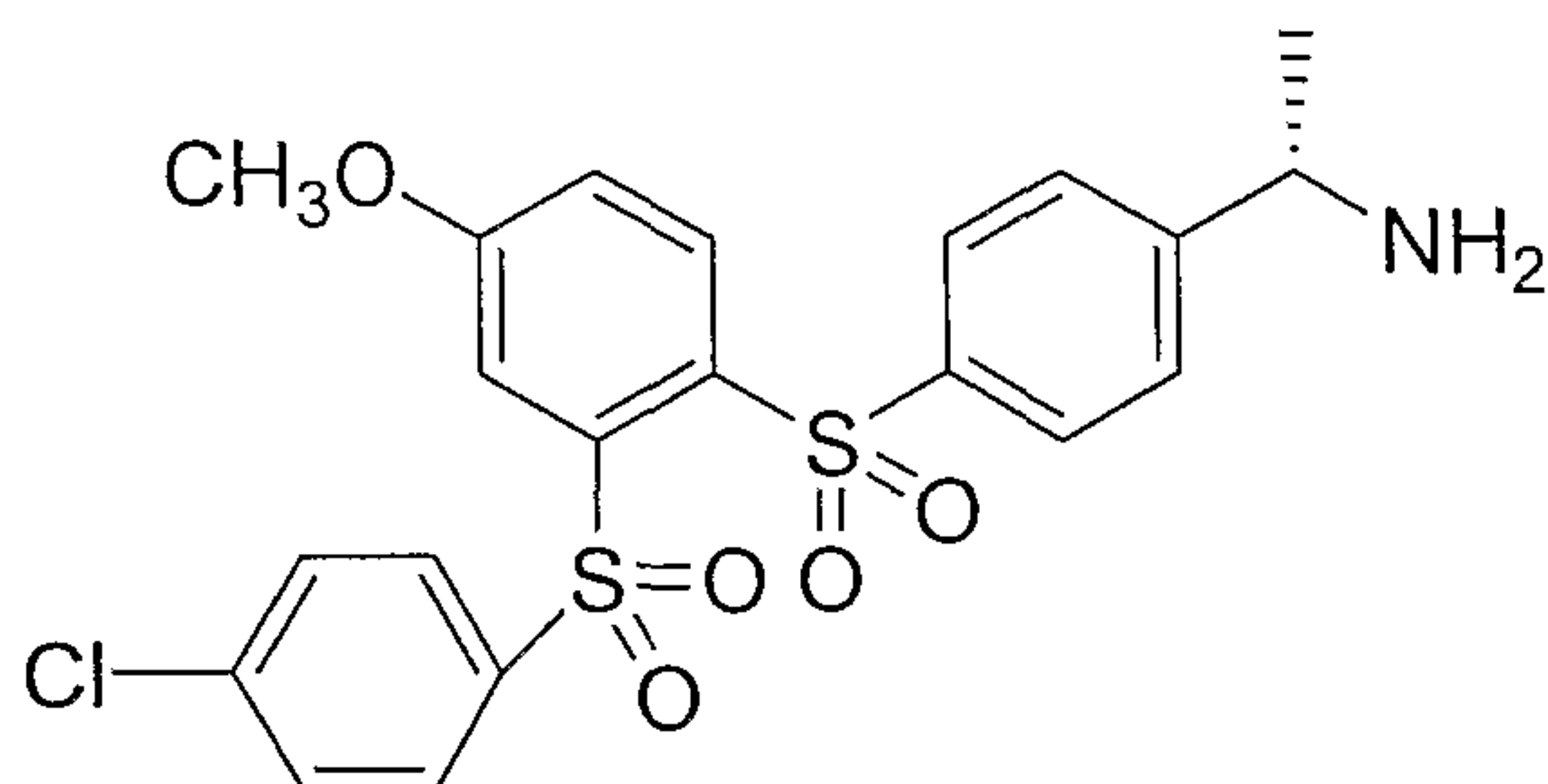
Compound 40
