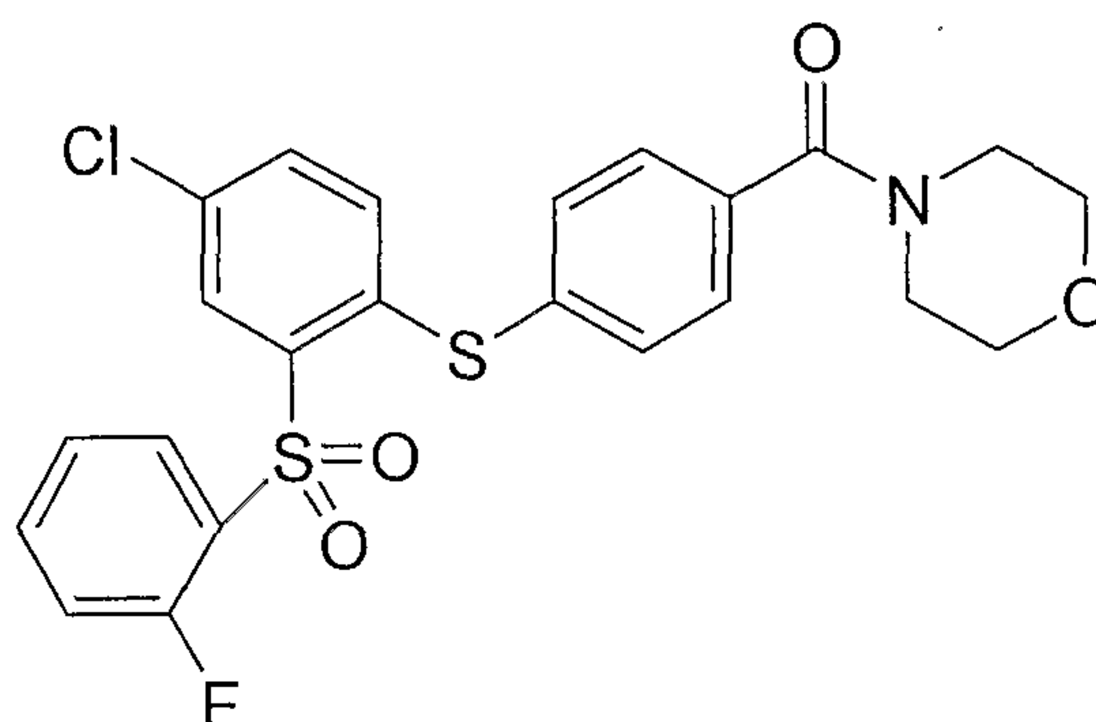
Compound XXVII
