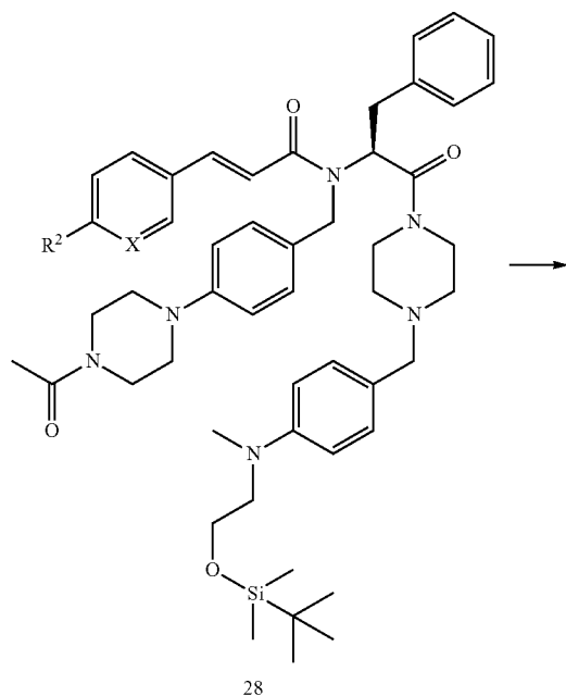
Scheme 16
