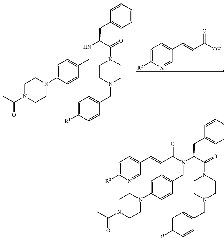
Scheme 10
