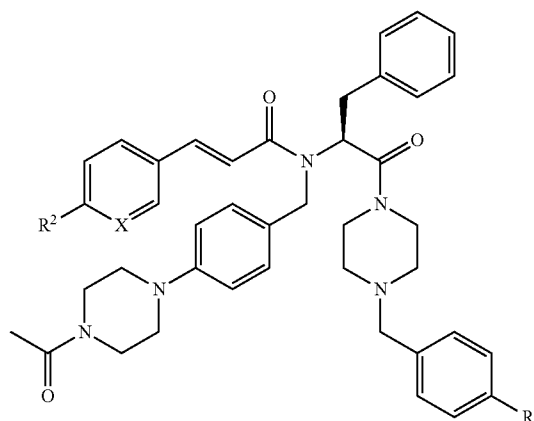
Formula I
