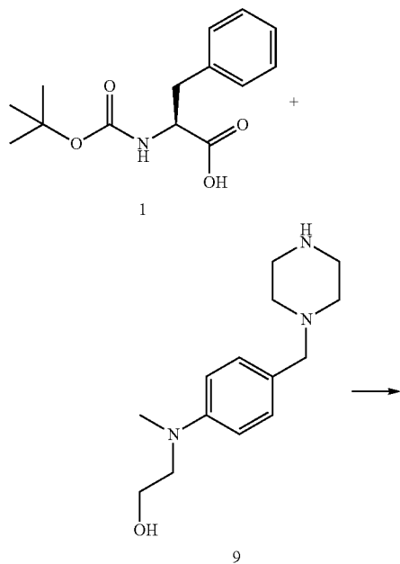
Scheme 11
