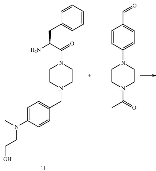
Scheme 13
