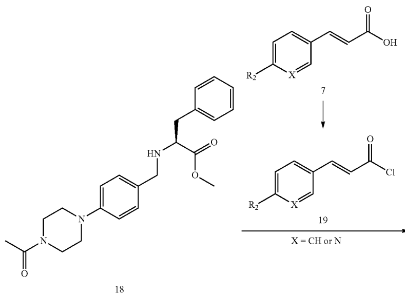
Scheme 18
