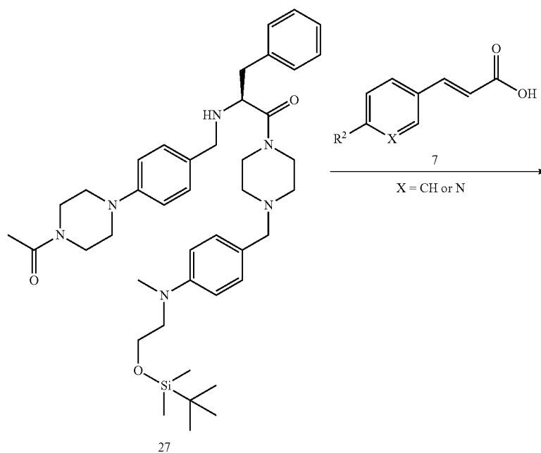
Scheme 15
