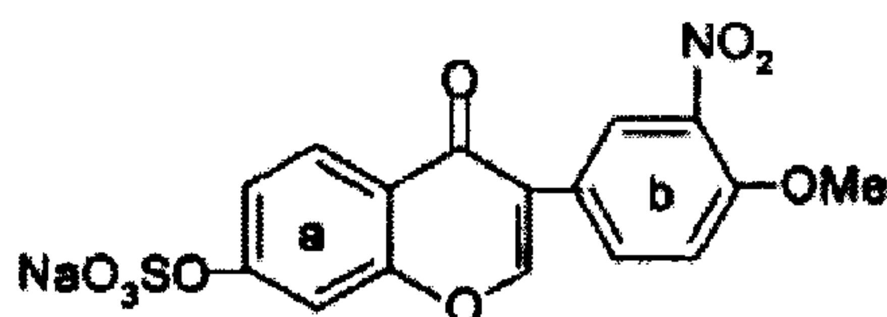
Example 3.6: 7-sodiosulfooxy-3'-nitro-4'-methoxyisoflavone
