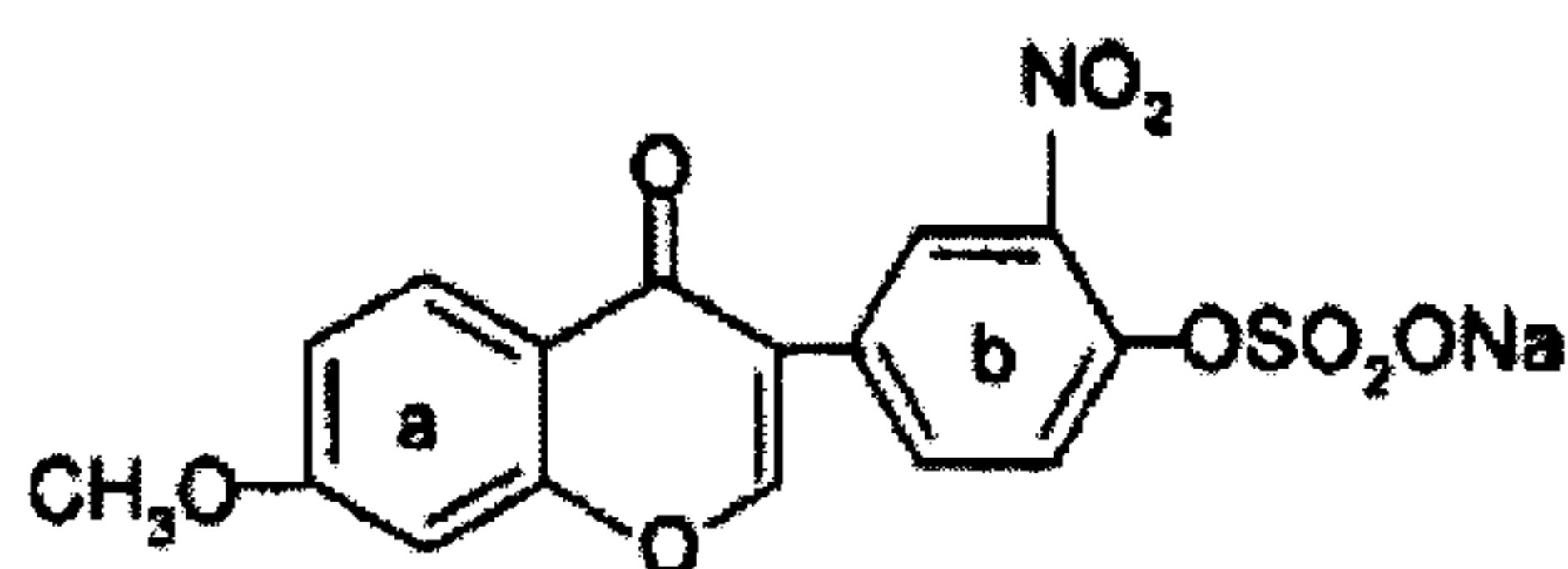
Example 3.6: 7-sodiosulfooxy-3'-nitro-4'-methoxyisoflavone
