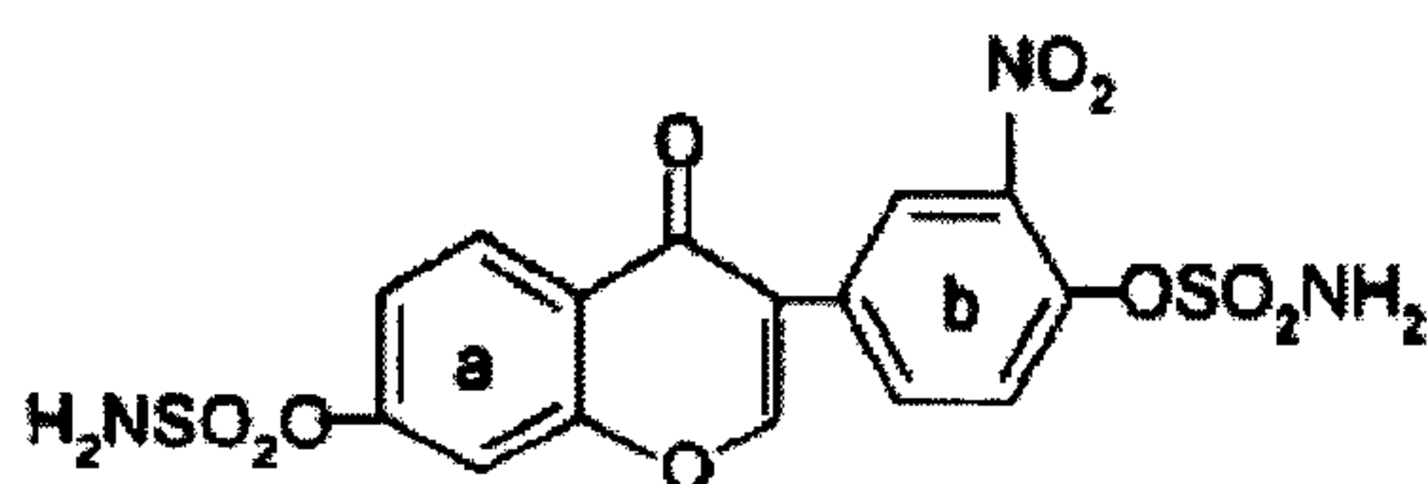
Example 3.8: 7,4'-disulfamoyloxy-3'-nitroisoflavone
