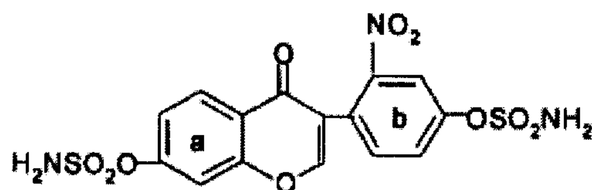
Example 3.8: 7,4'-disulfamoyloxy-3'-nitroisoflavone
