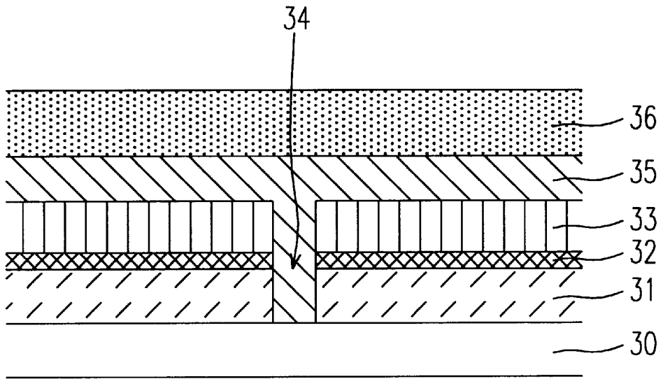
Fig. 3(a)(PRIOR ART)
