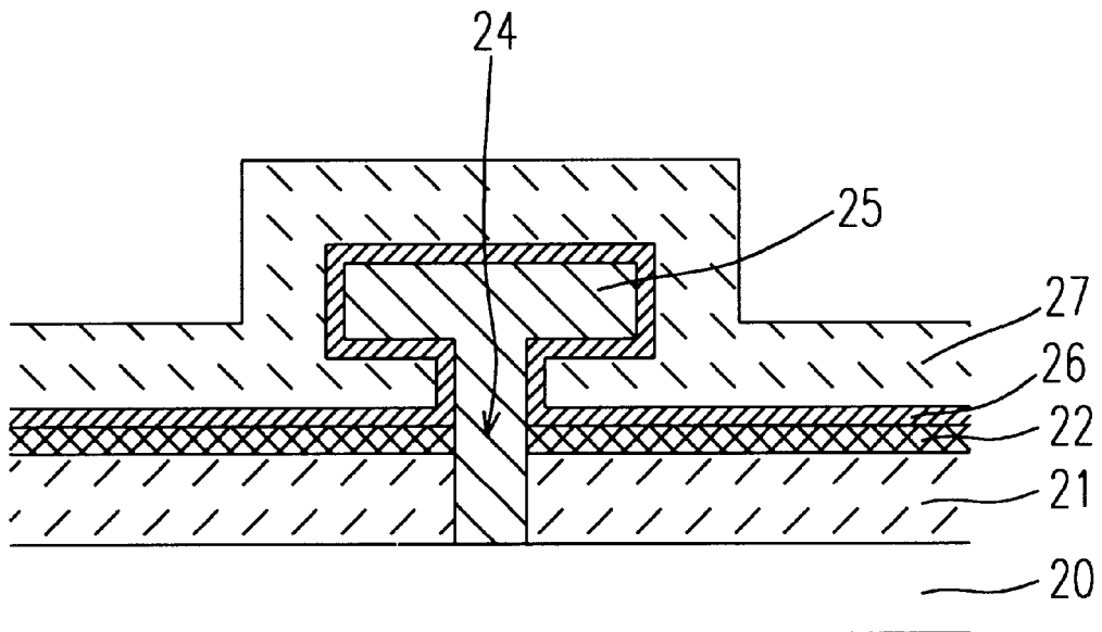
Fig. 2(b)(PRIOR ART)
