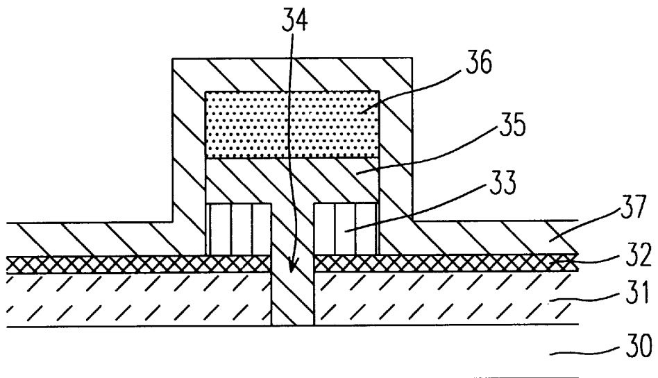
Fig. 3(b)(PRIOR ART)
