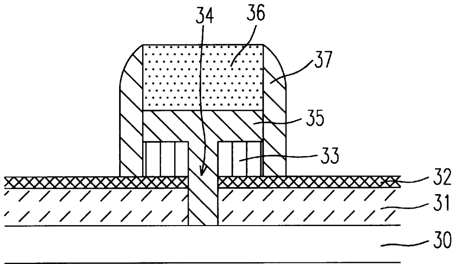
Fig. 3(c)(PRIOR ART)
