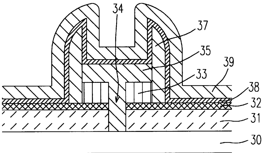
Fig. 3(d)(PRIOR ART)
