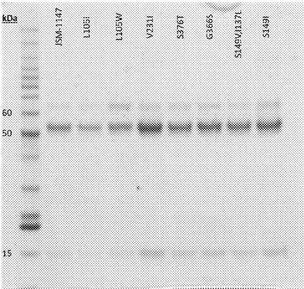
Cavity mutations
