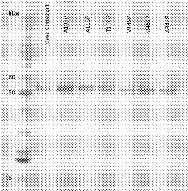
Proline mutations
