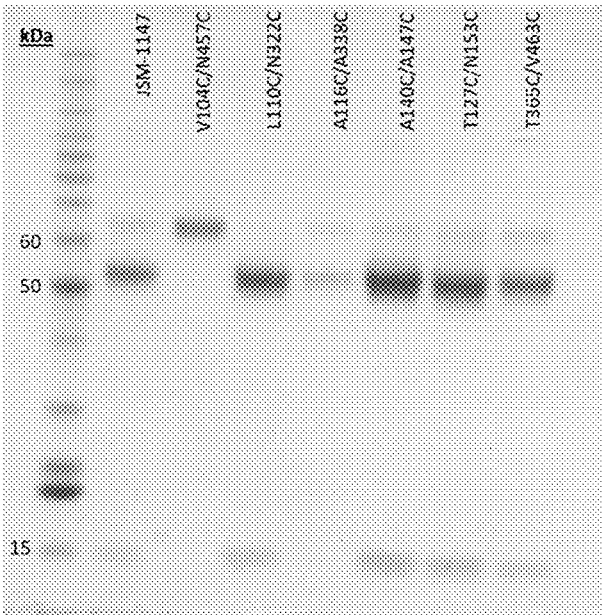
Disulfide mutations
