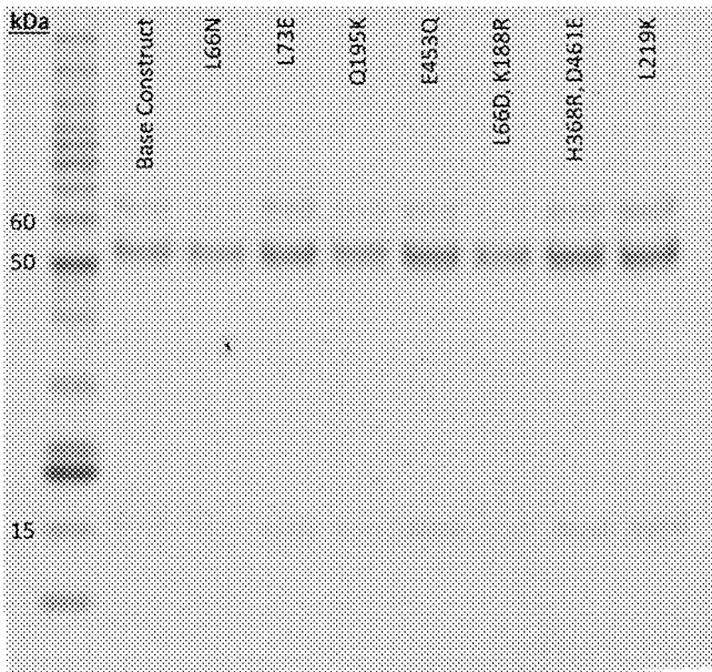
Electrostatic mutations
