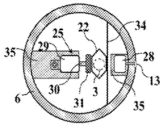
Full Open Position
