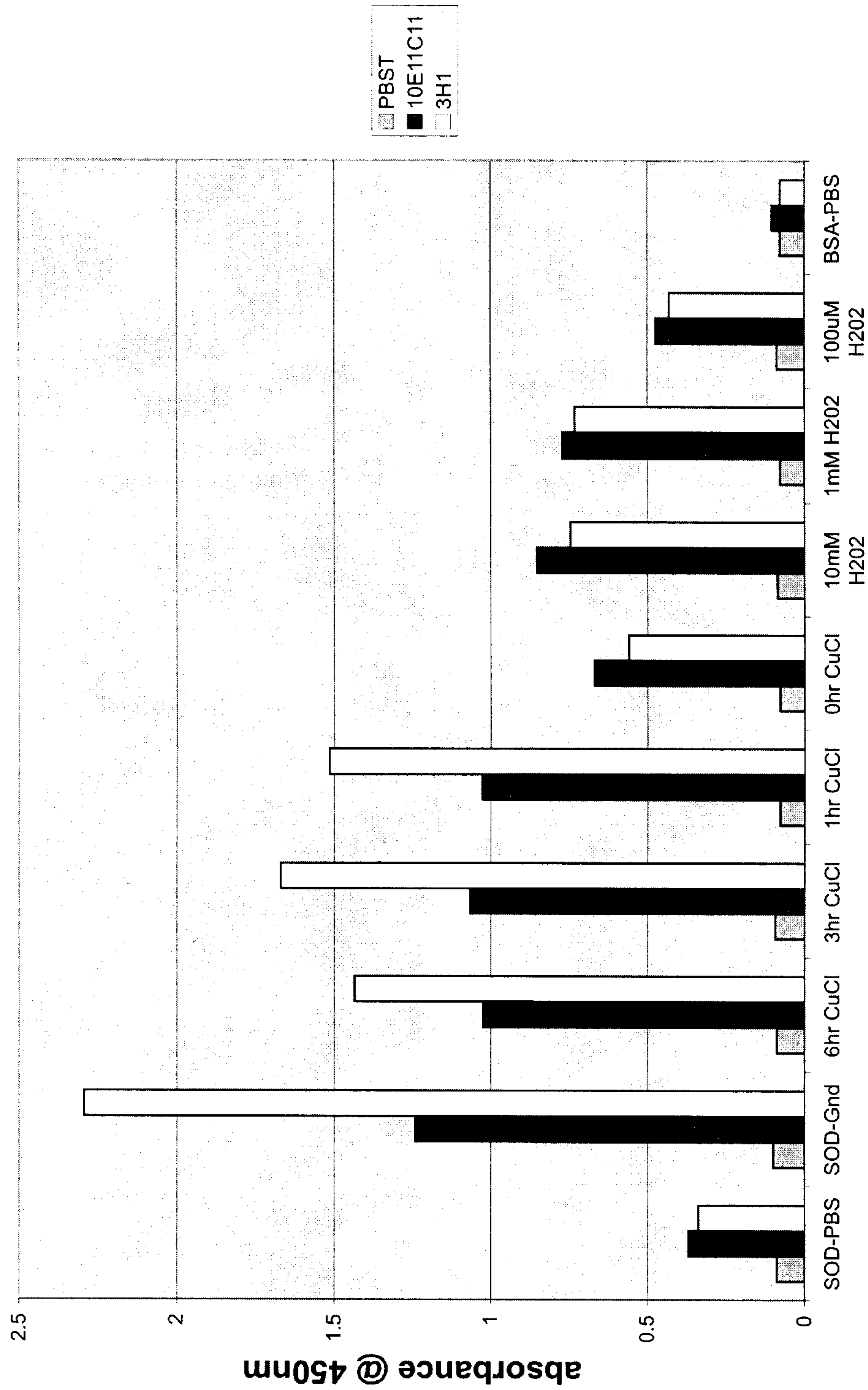
Oxidizing Condition
