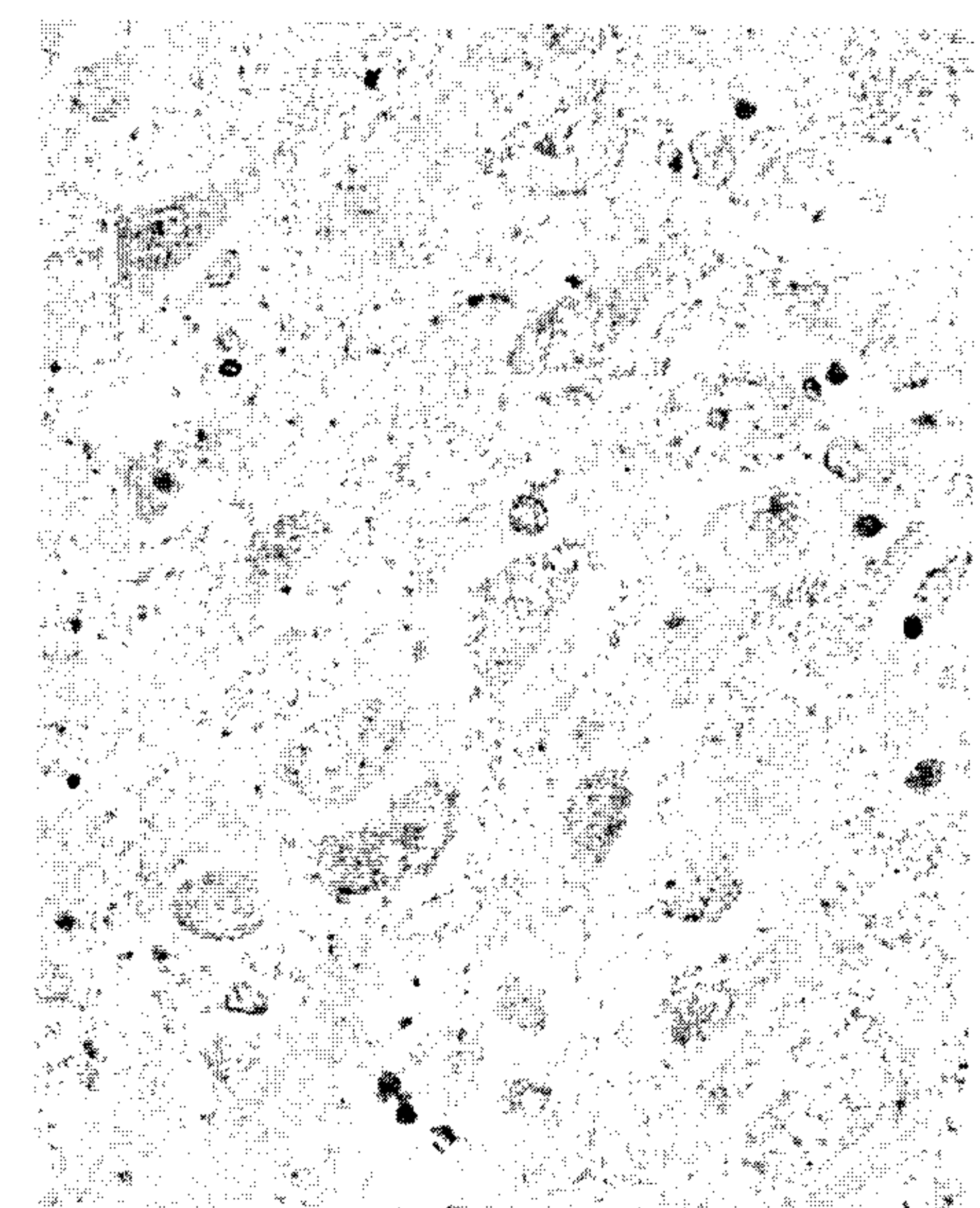
Normal Hippocampus
