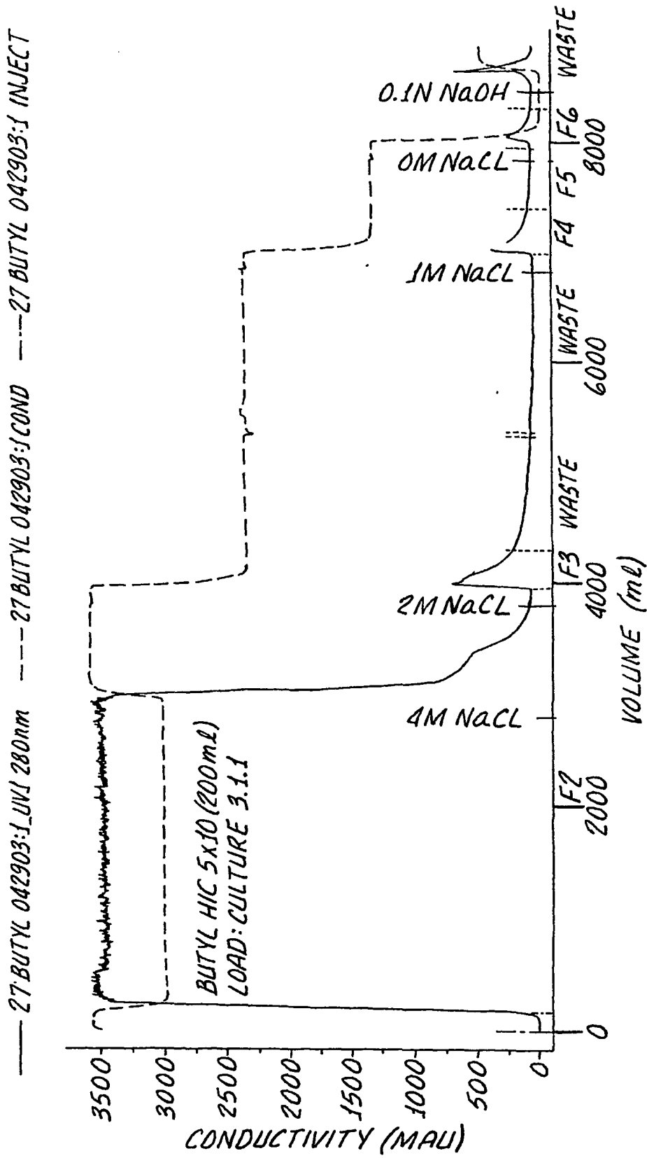
CHROMATOGRAM OF BUTYL SEPHAROSE FF CHROMATOGRAPHY
