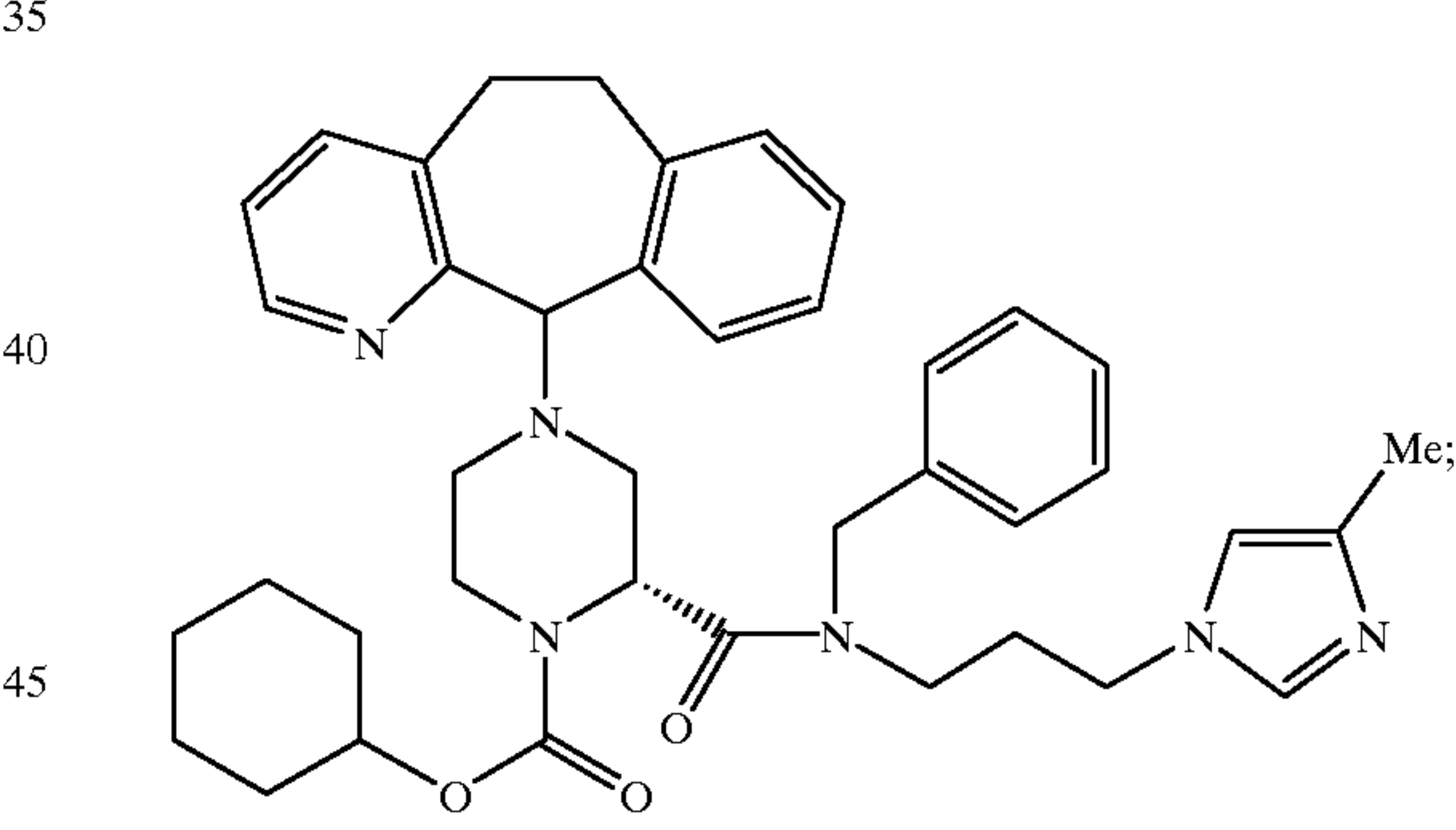
Example 373 (Isomer B)
