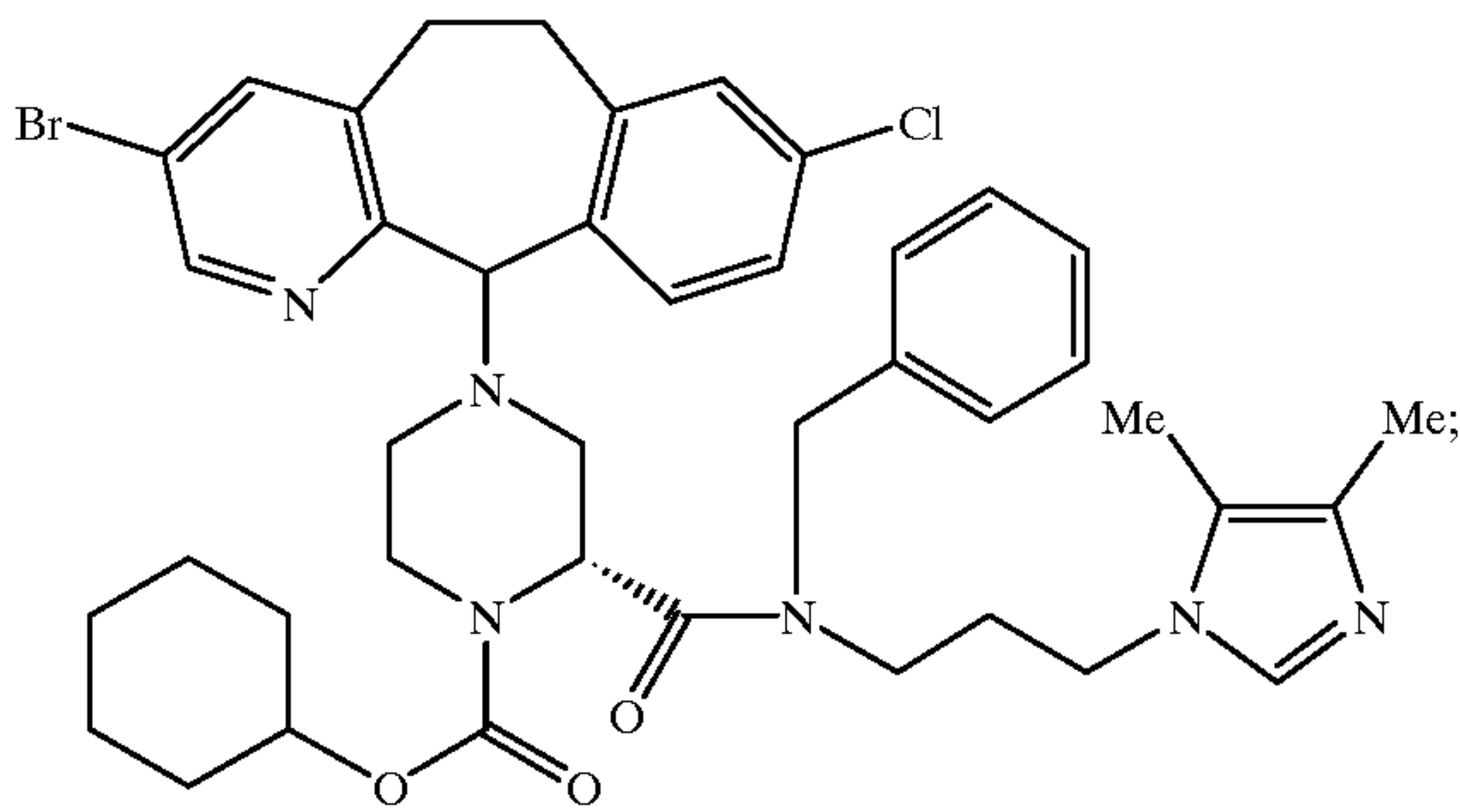
Example 378 (Isomer B)
