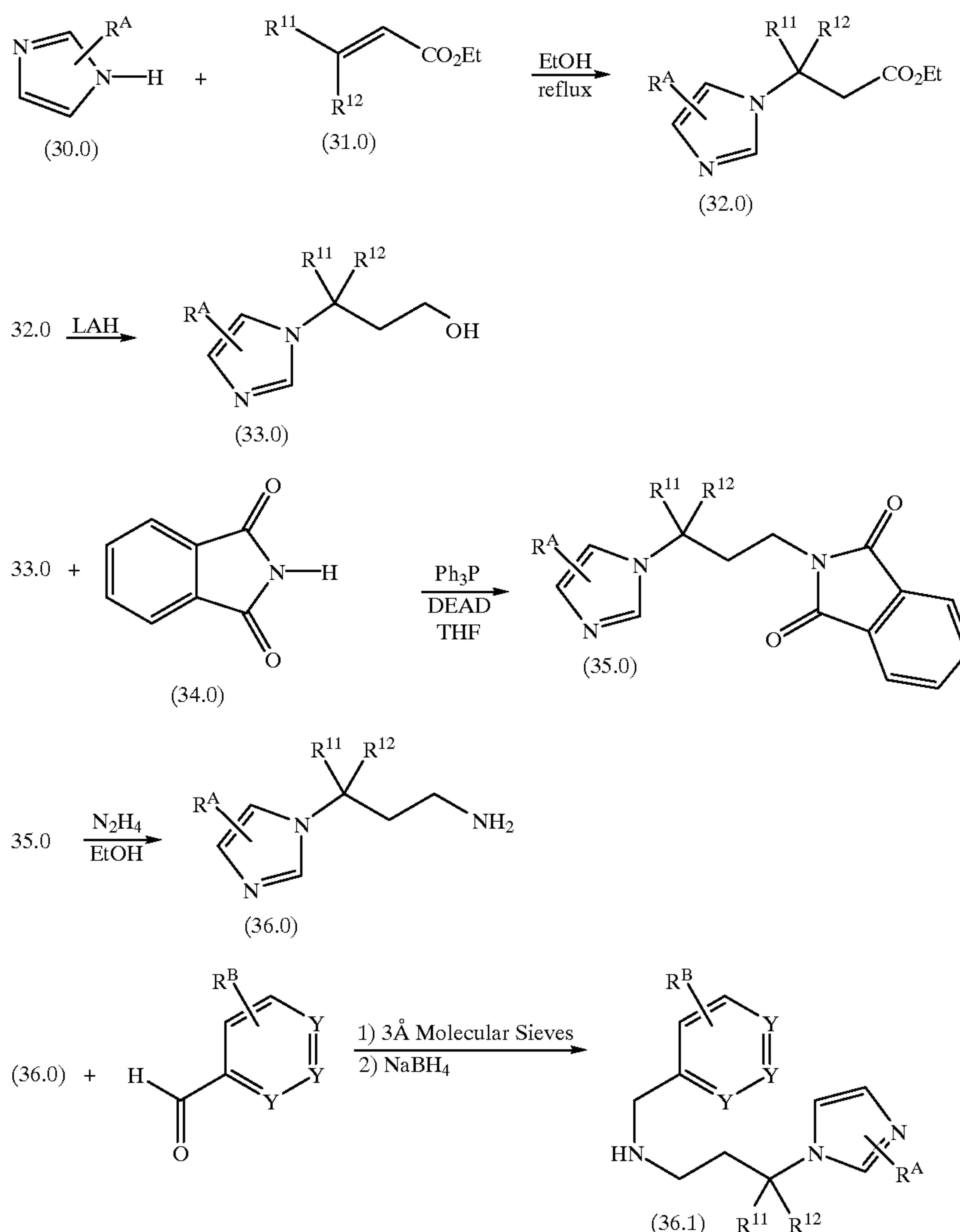
Reaction Scheme 1 (n is 1)
