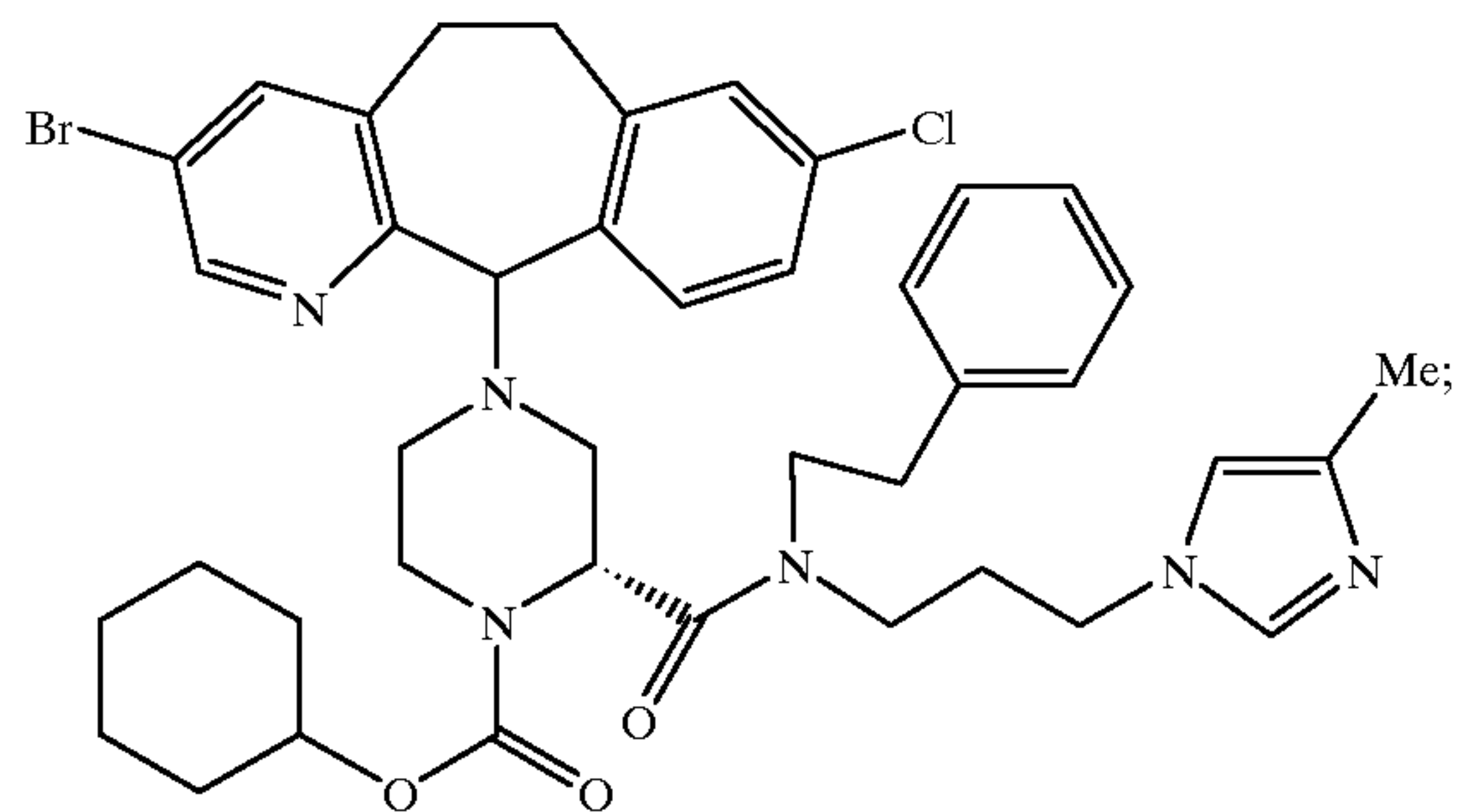
Example 379 (Isomer A)
