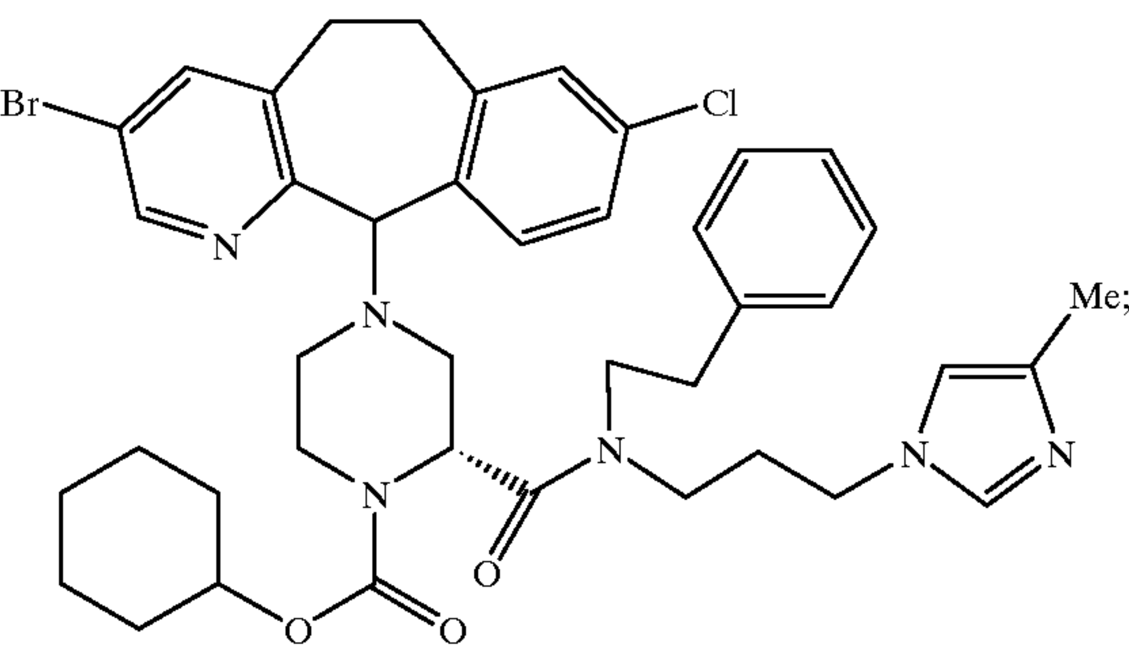
Example 380 (Isomer B)
