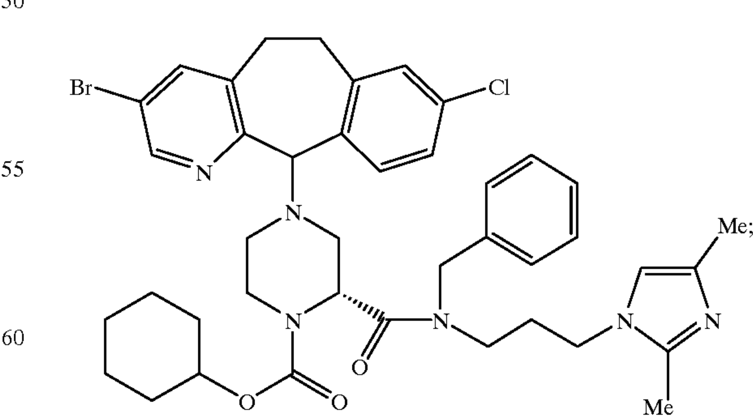
Example 375 (Isomer A)
