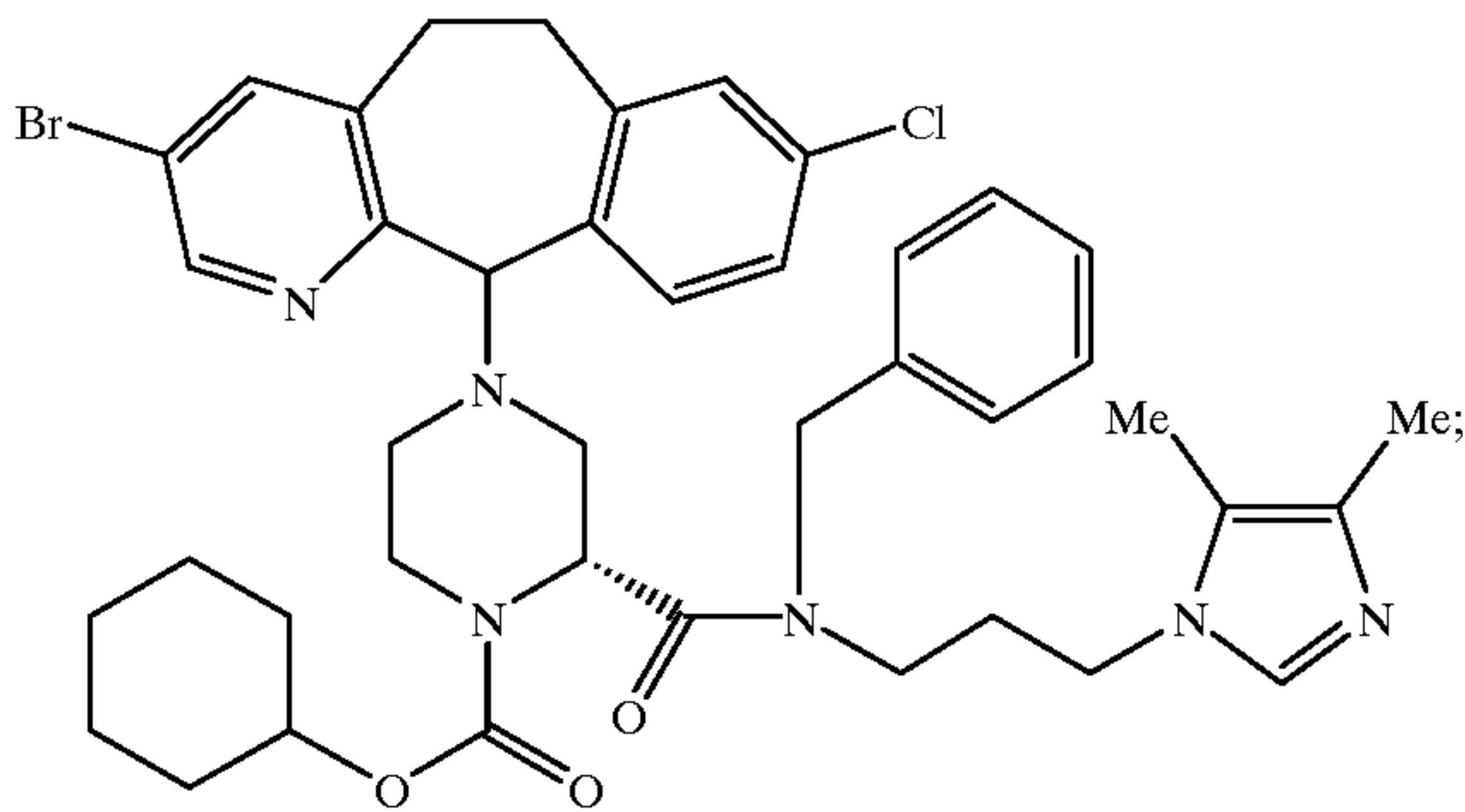
Example 377 (Isomer A)
