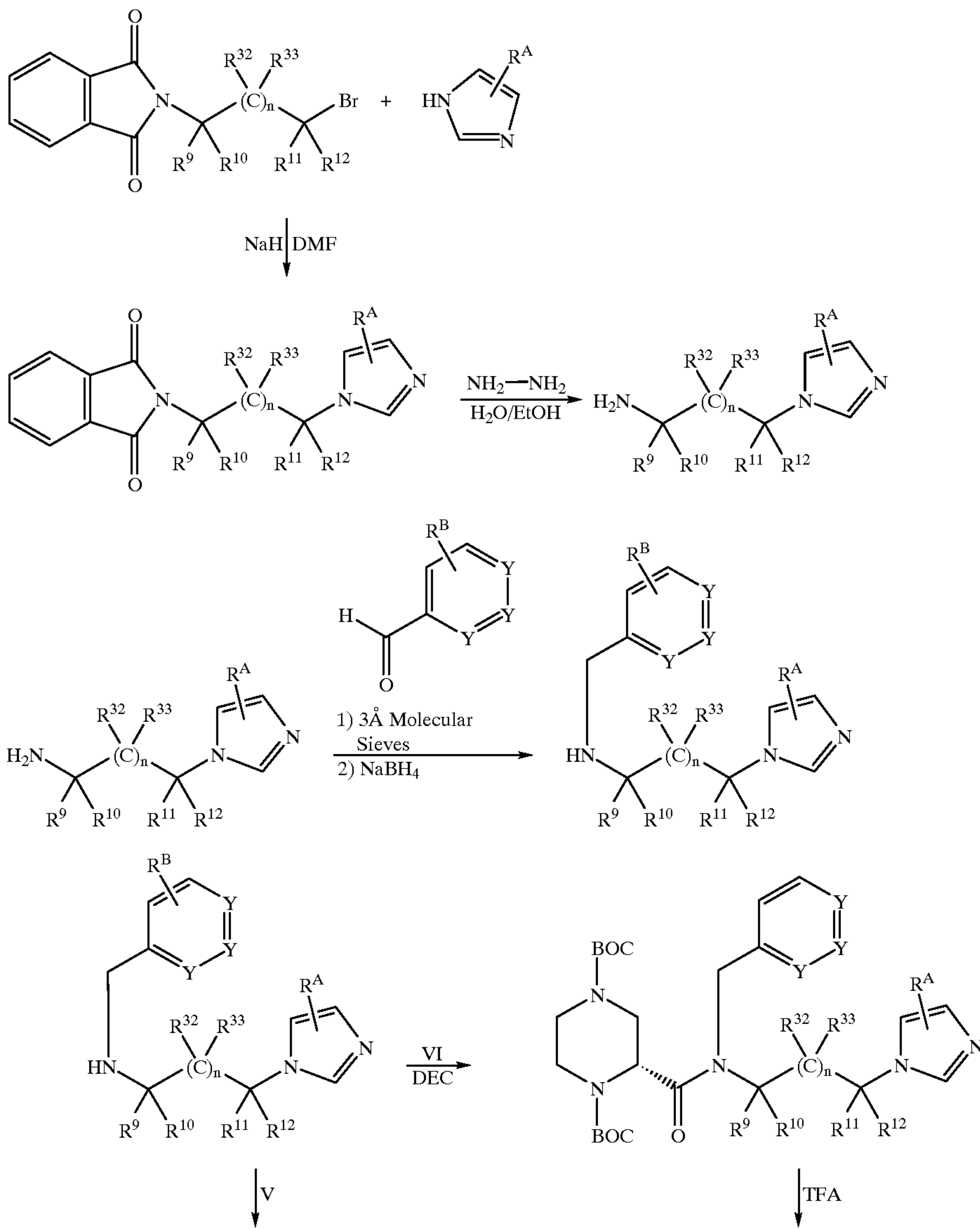
Reaction Scheme 4 (n is 1–5)
