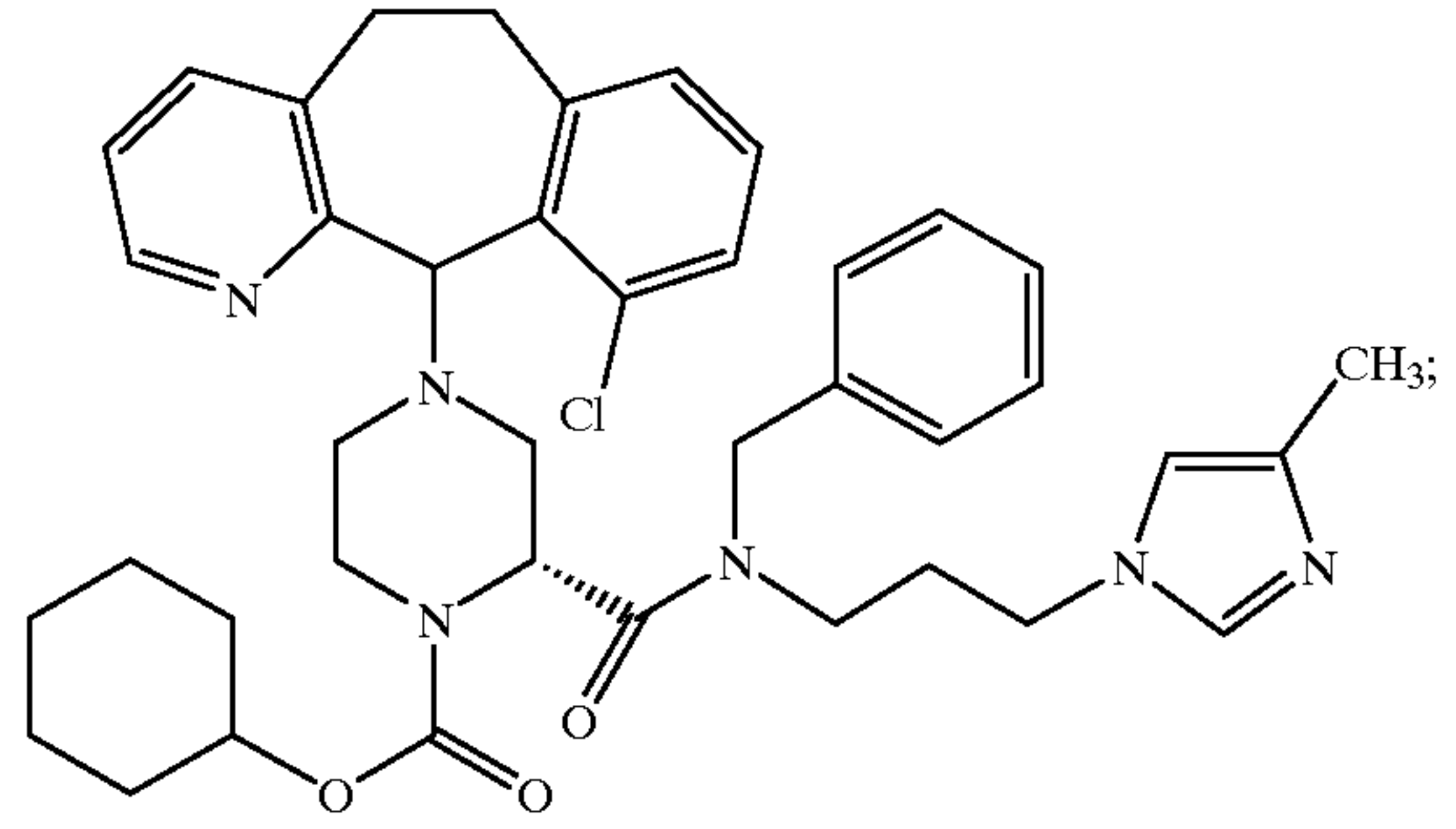
Example 383 (Isomer A)
