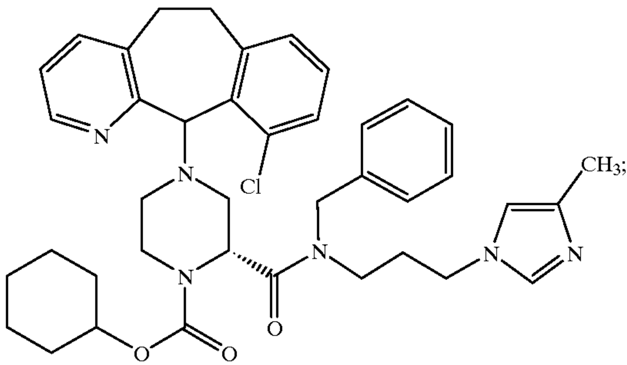
Example 384 (Isomer B)
