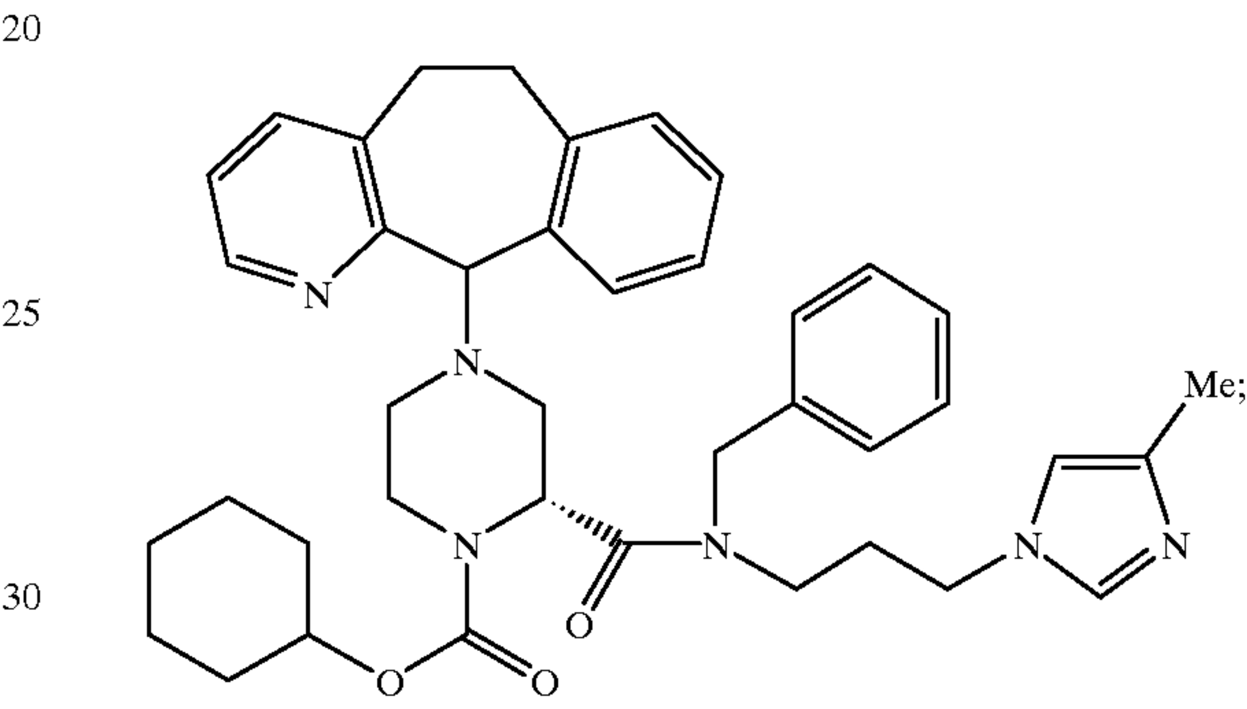
Example 372 (Isomer A)
