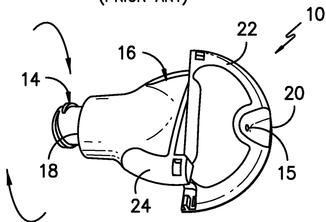
FIG. -2- (PRIOR ART)
