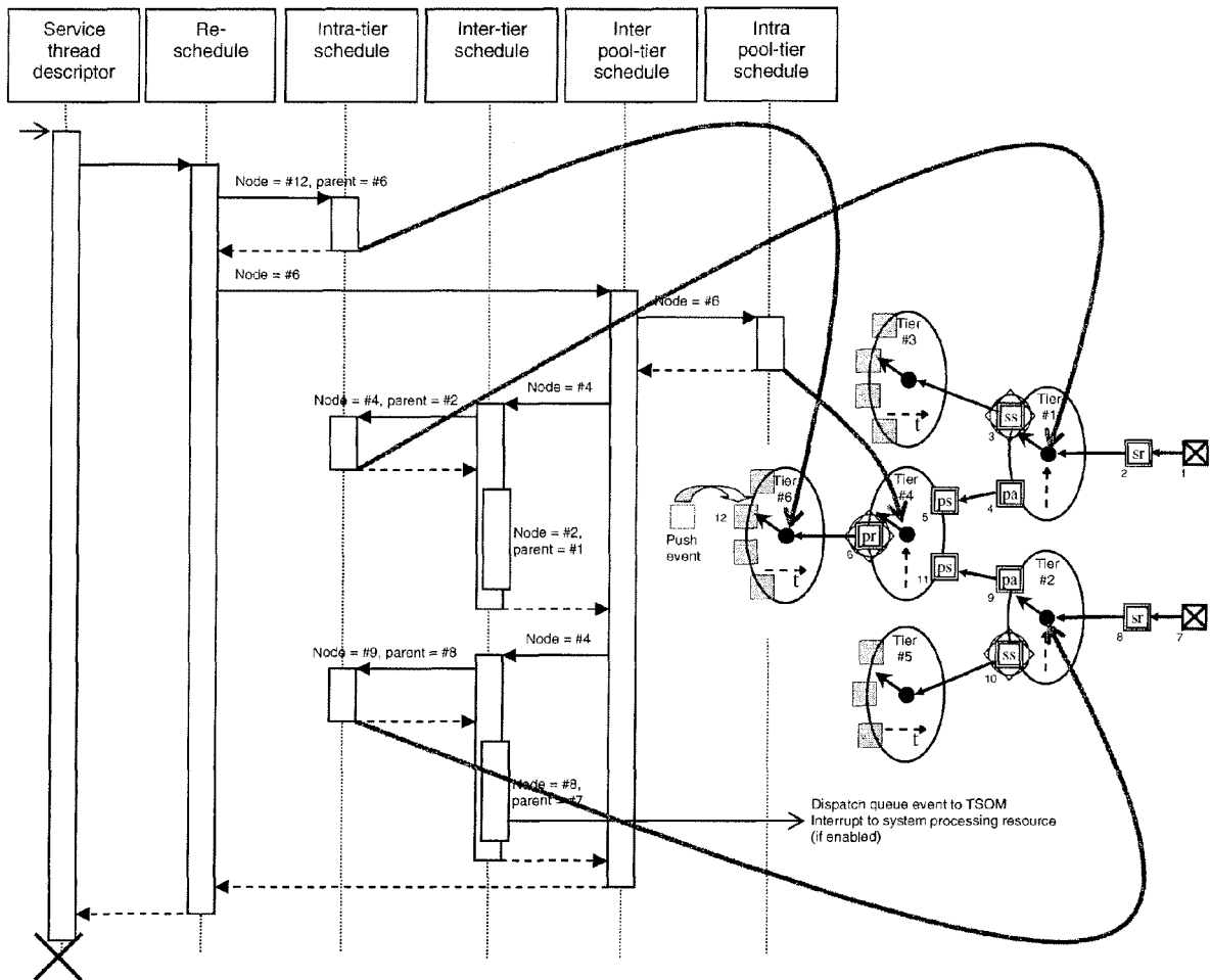
Figure 70: A pool based scheduling hierarchy sequence diagram
