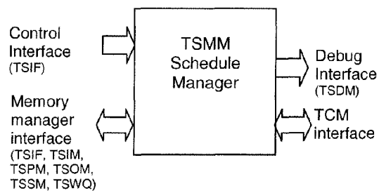
Figure 71: TSM primary IO
