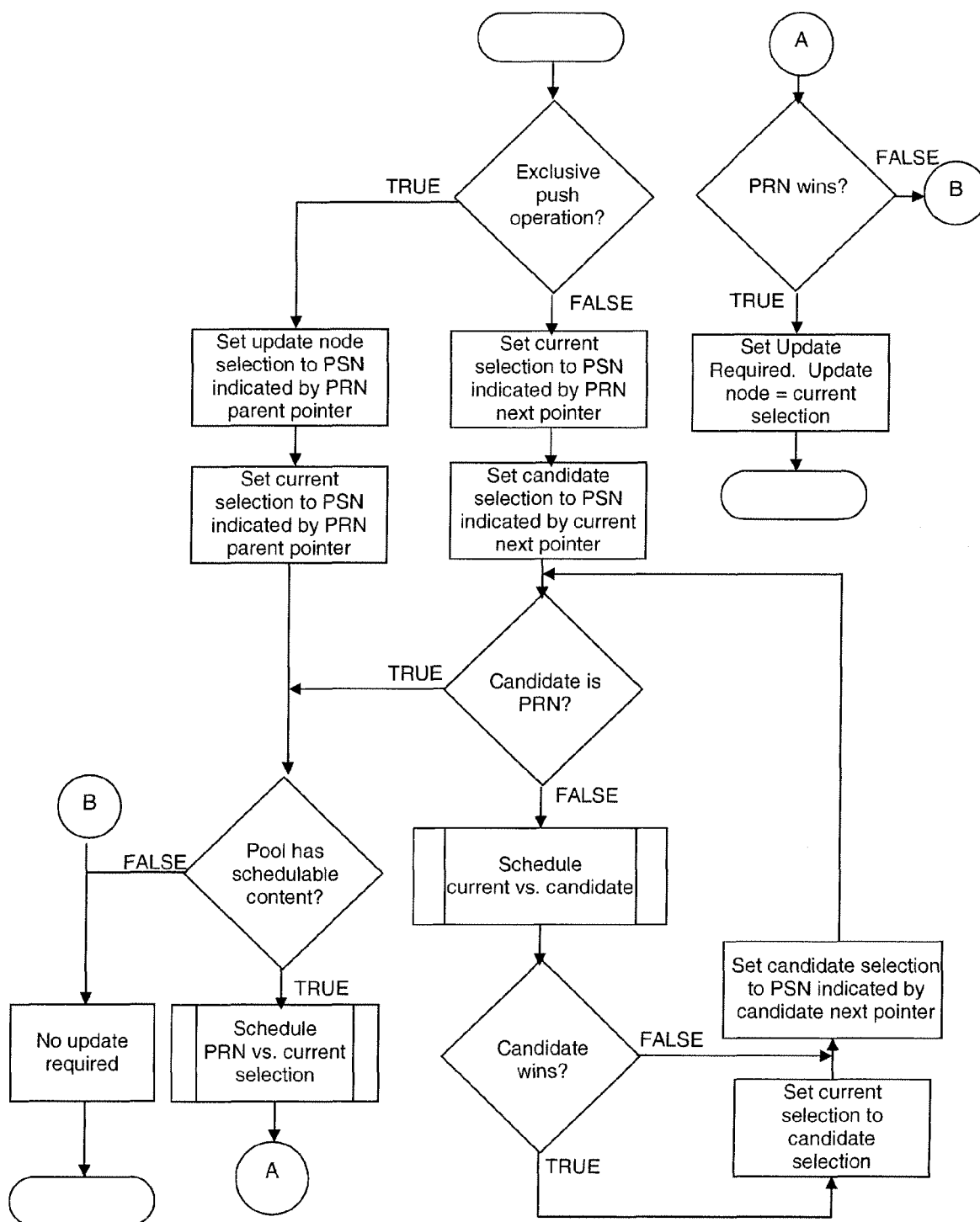
Figure 67: Intra-pool tier scheduler processing
