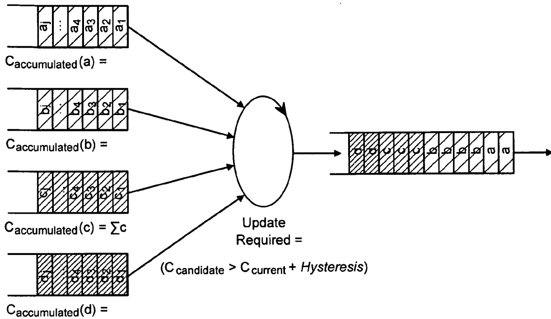
Figure 32: Scheduler grouping for minimal context thrashing
