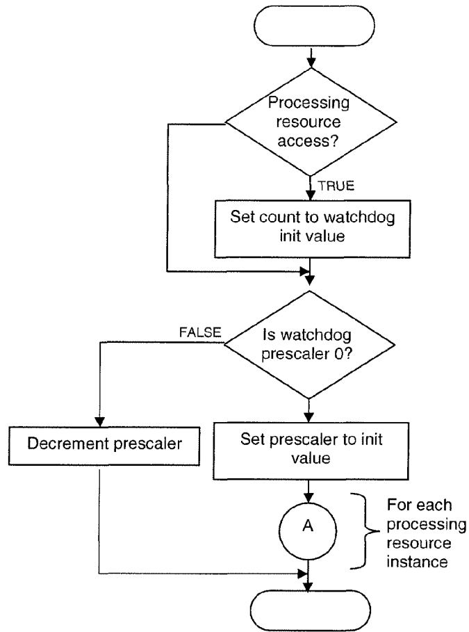
Figure 44: Watchdog interrupt control per cycle
