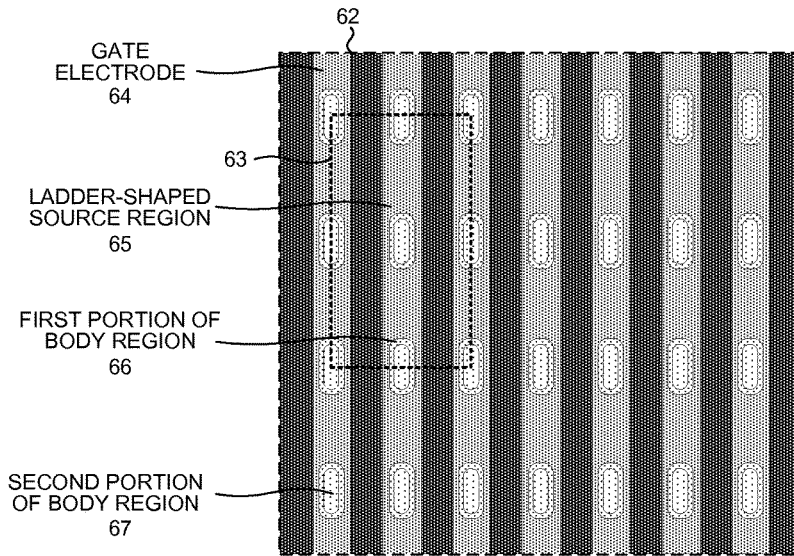
EXPANDED TOP-DOWN VIEW OF RECTANGLE 62 OF FIG. 16
