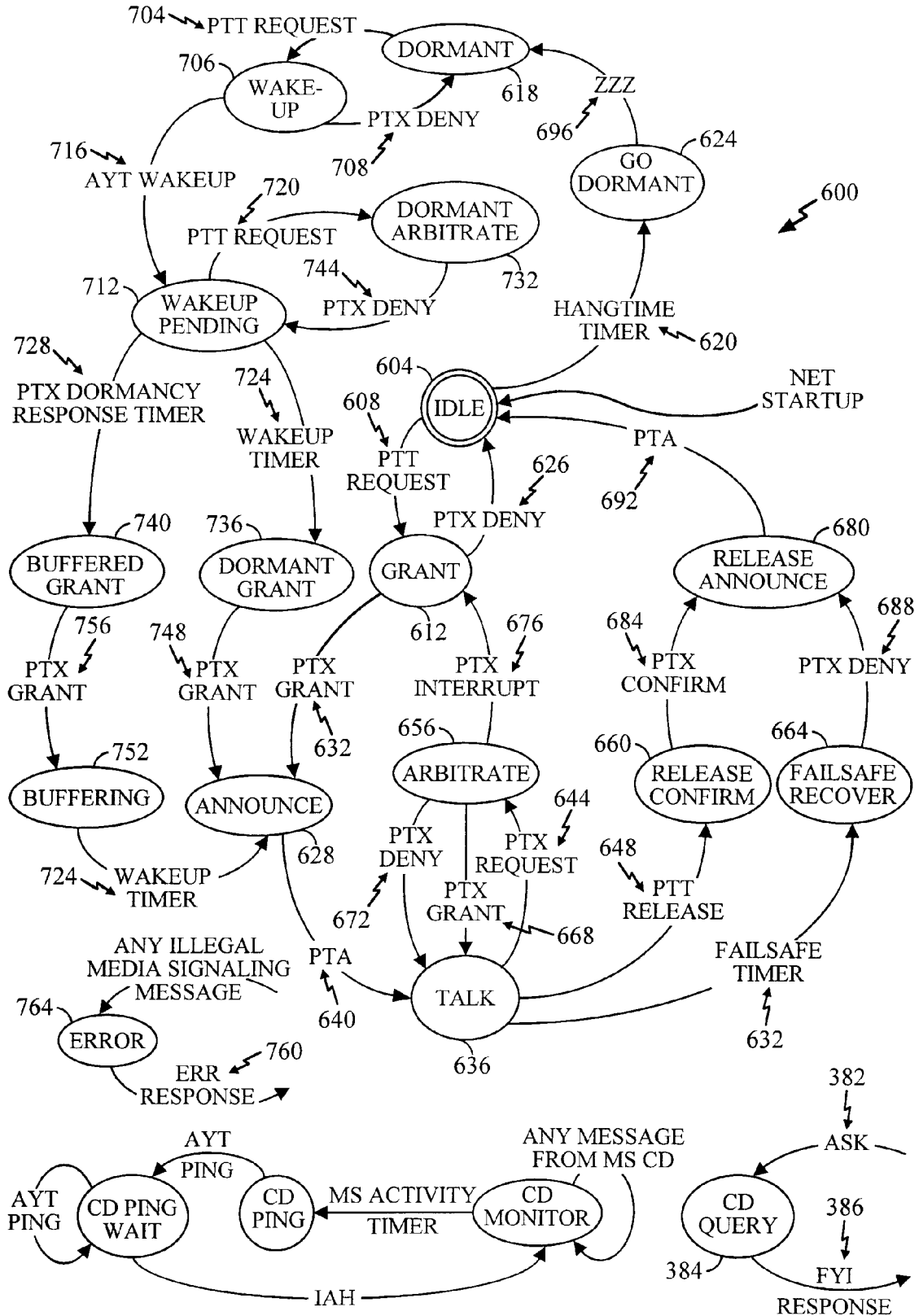
FIG. 15 MEDIA SIGNALING STATE DIAGRAM
