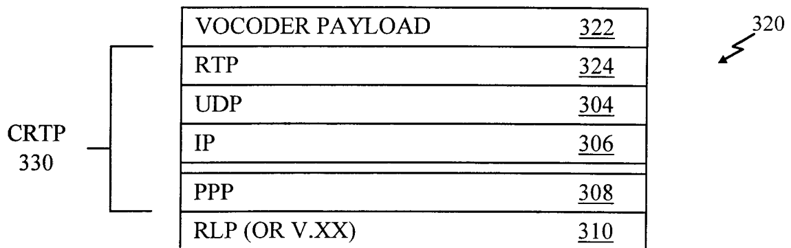
RTP VOICE MEDIA PROTOCOL STACK
