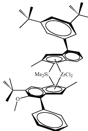
rac-anti-Me 2 Si(2-Me-4-(3,5-di-tBuPh)-7-Me-Ind)(2-Me-4-Ph-5-OMe-6-tBu-Ind)ZrCl 2
