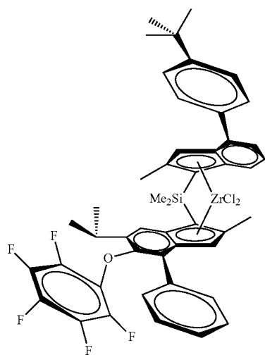
rac-anti-Me 2 Si(2-Me-4-(p-tBuPh)-Ind)(2-Me-4-Ph-5-OC 6 F 5 -6-iPr-Ind)ZrCl 4
