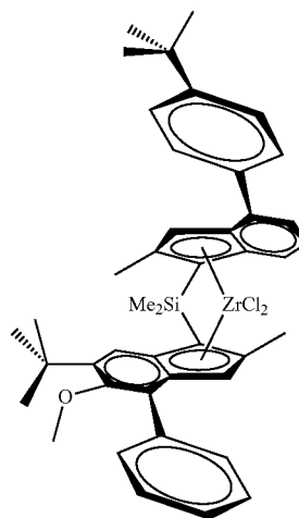
rac-anti-Me 2 Si(2-Me-4-(p-tBuPh)-Ind)(2-Me-4-Ph-5-OMe-6-tBu-Ind)ZrCl 2
