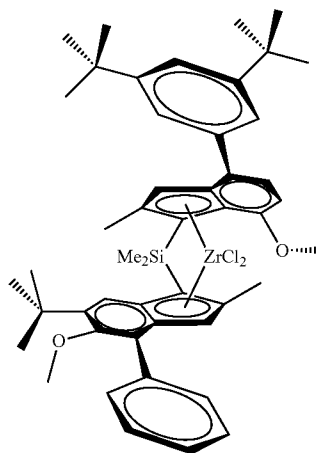
rac-anti-Me 2 Si(2-Me-4-(3,5-di-tBuPh)-7-OMe-Ind)(2-Me-4-Ph-5-OMe-6-tBu-Ind)ZrCl 2
