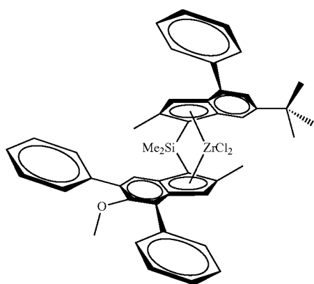
rac-anti-Me 2 Si(2-Me-4-Ph-6-tBu-Ind)(2-Me-4,6-di-Ph-5-OMe-Ind)ZrCl 2
