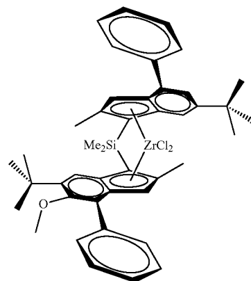
rac-anti-Me 2 Si(2-Me-4-Ph-6-tBu-Ind)(2-Me-4-Ph-5-OMe-6-tBu-Ind)ZrCl 2
