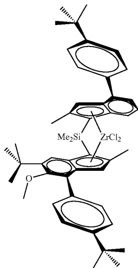
rac-anti-Me 2 Si(2-Me-4-(p-tBuPh)-Ind)(2-Me-4-(4-tBuPh)-5-OMe-6-tBu-Ind)ZrCl 2
