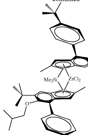
rac-anti-Me 2 Si(2-Me-4-(p-tBuPh)-Ind)(2-Me-4-Ph-5-OiBu-6-tBu-Ind)ZrCl 2
