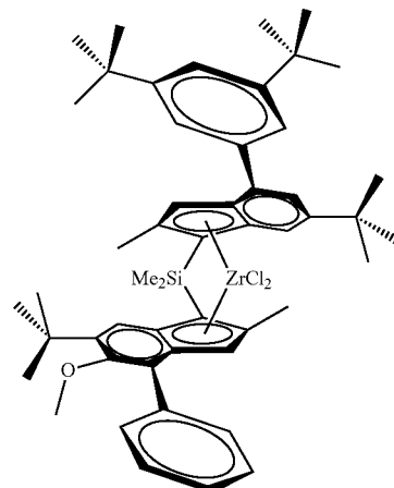
rac-anti-Me 2 Si(2-Me-4-(3,5-di-tBuPh)-6-tBu-Ind)(2-Me-4-Ph-5-OMe-6-tBu-Ind)ZrCl 2
