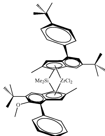
rac-anti-Me 2 Si(2-Me-4-(p-tBuPh)-6-tBu-Ind)(2-Me-4-Ph-5-OMe-6-tBu-Ind)ZrCl 2
