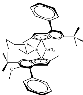
rac-anti-Me(CyHex)Si(2-Me-4-Ph-6-tBu-Ind)(2-Me-4-Ph-5-OMe-6-tBu-Ind)ZrCl 2
