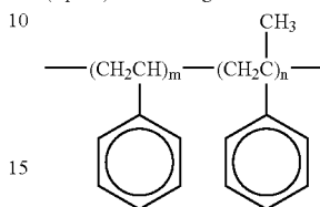
(Cpd-6) Color-image stabilizer
