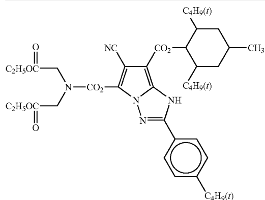
(ExC-5) Cyan coupler
