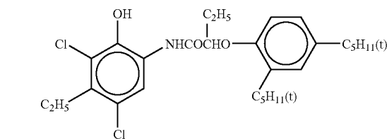
Coupler for comparison C1
