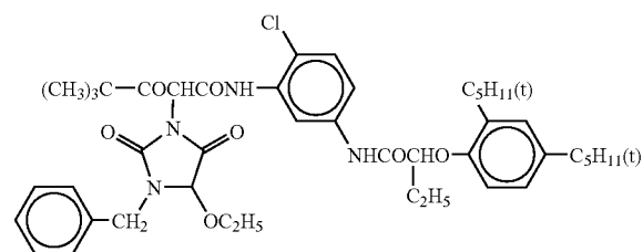
Coupler for comparison C1
