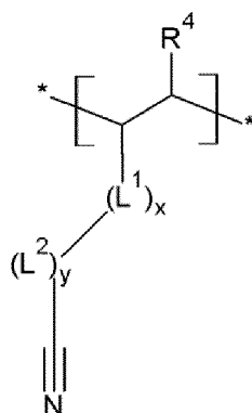
[Chemical Formula 4]
