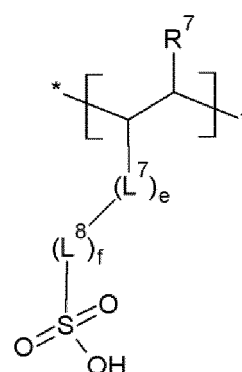
[Chemical Formula 7]
