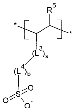
[Chemical Formula 5]
