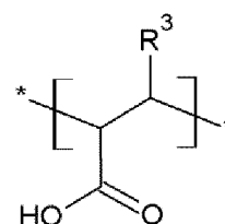
[Chemical Formula 3]
