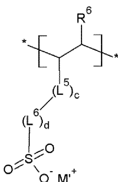
[Chemical Formula 6]
