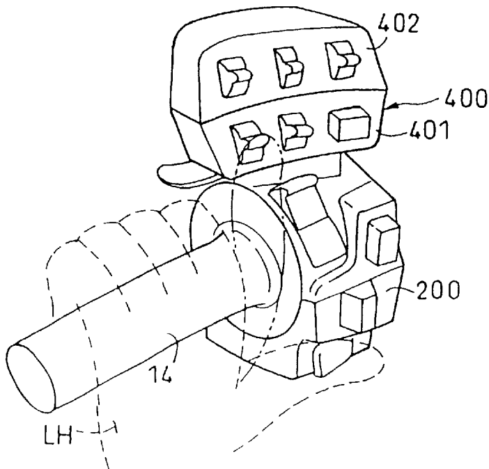
FIG. 6 BACKGROUND ART
