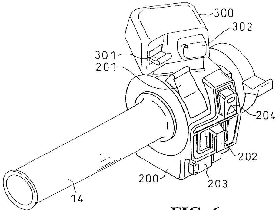
FIG. 6 BACKGROUND ART
