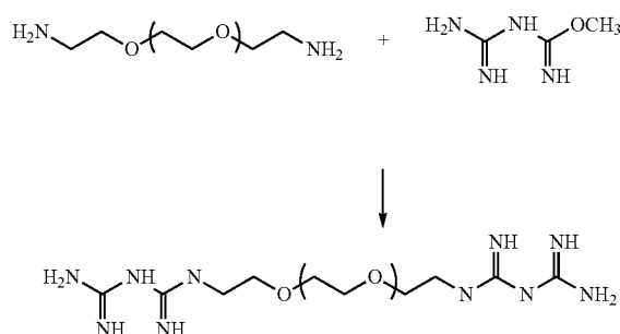
Reaction Scheme V:
