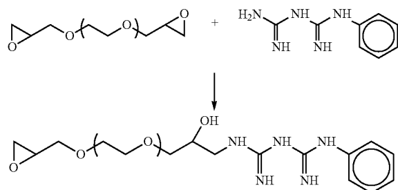
Reaction Scheme IV:
