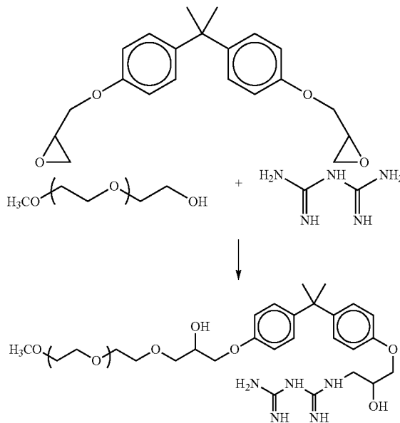
Reaction Scheme VI:
