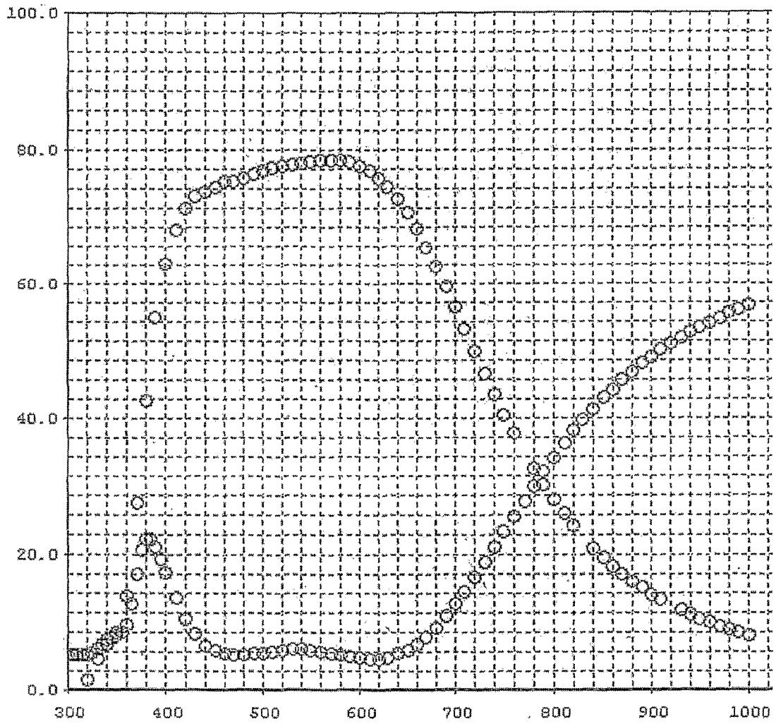
Reflectance (%) and Transmittance (%) vs Wavelength
