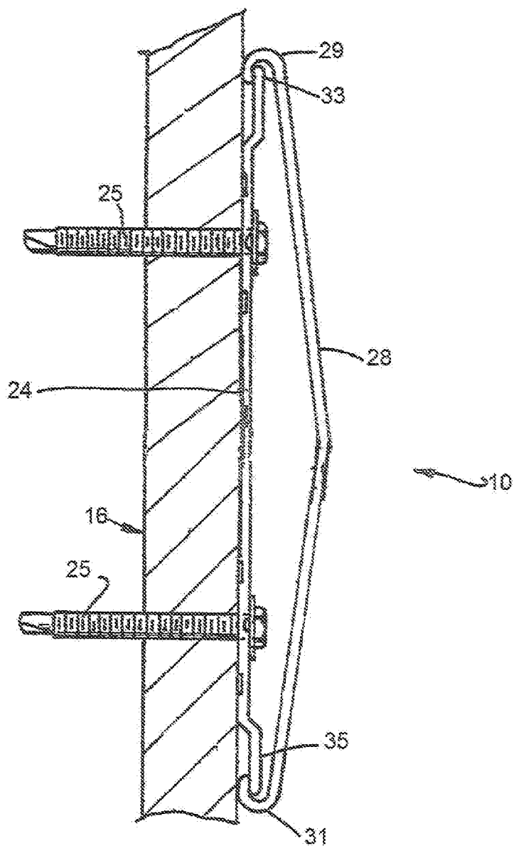
FIG. 24 PRIOR ART
