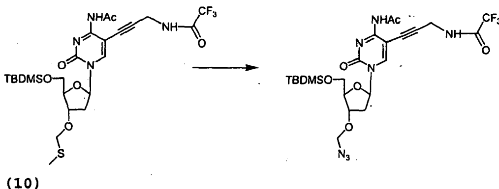
4- N -Acetyl-3'- O -(azidomethyl)-5'- O -(tert-butyldimethylsilyl)-5-[3-(2,2,2-trifluoroacetamide)-prop-1-ynyl]-2'-deoxycytidine (10).
