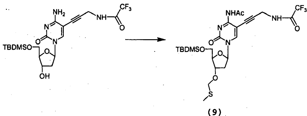
4- N -Acetyl-5'- O -(tert-butyldimethylsilyl)-3'- O -(methylthiomethyl)-5-[3-(2,2,2-trifluoroacetamide)-prop-1-ynyl]-2'-deoxycytidine (9).
