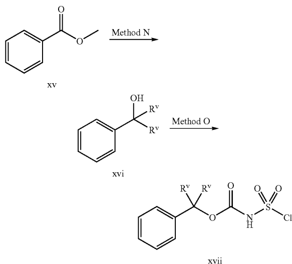
Scheme 3: General route for the synthesis of substituted-(chlorosulfonyl)-carbamates R''NHS(O)_2Cl
