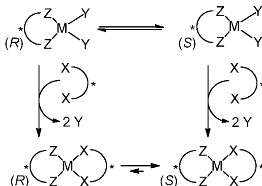
Scheme 2. Chemosensing and Chiral Induction with Stereodynamic Metal Complexes
