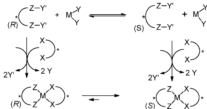
Scheme 3. Chemosensing and Chiral Induction with Stereodynamic Metal Complexes
