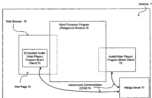
Wedge Server and Event Client Programs
