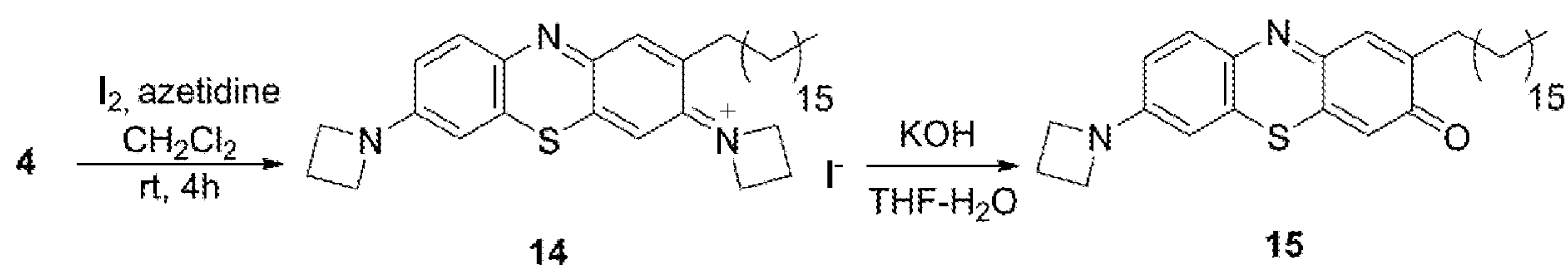
Scheme 6
