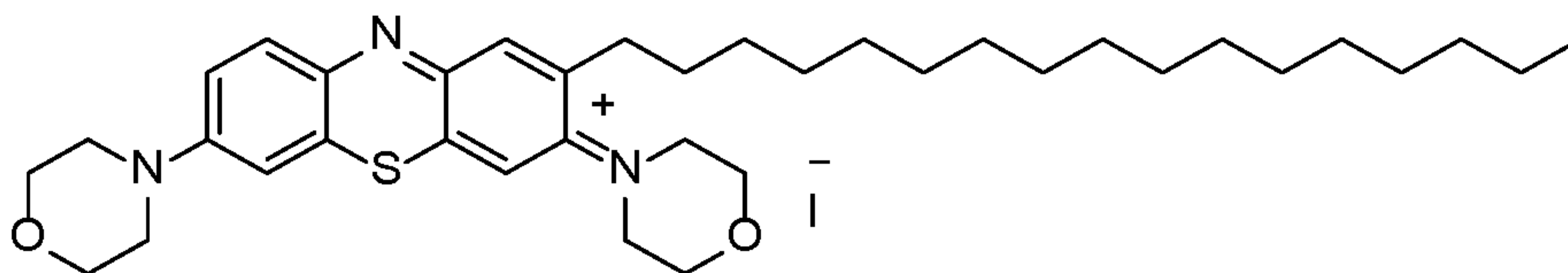
4-(2-heptadecyl-7-morpholino-3H-phenothiazin-3-ylidene)morpholin-4-ium iodide (10)
