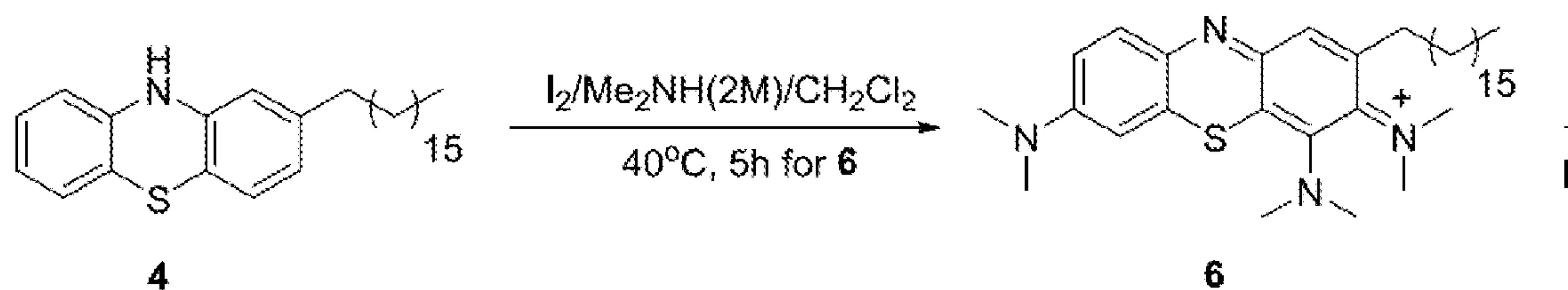
Scheme 2
