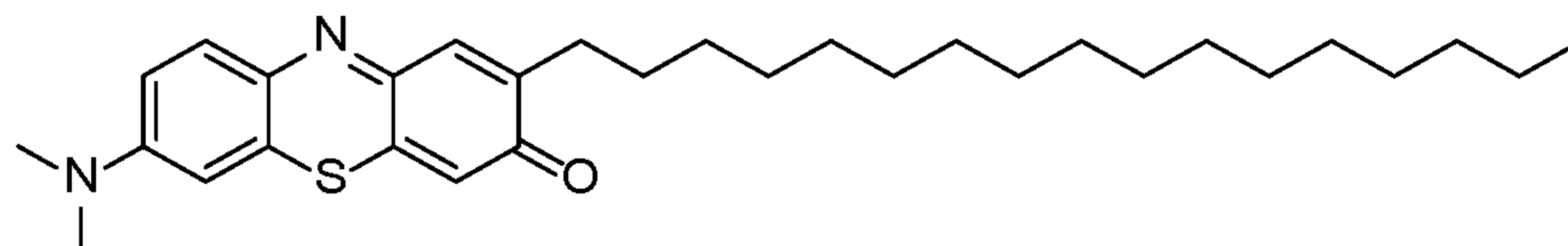
7-(dimethylamino)-2-heptadecyl-3H-phenothiazin-3-one (7)
