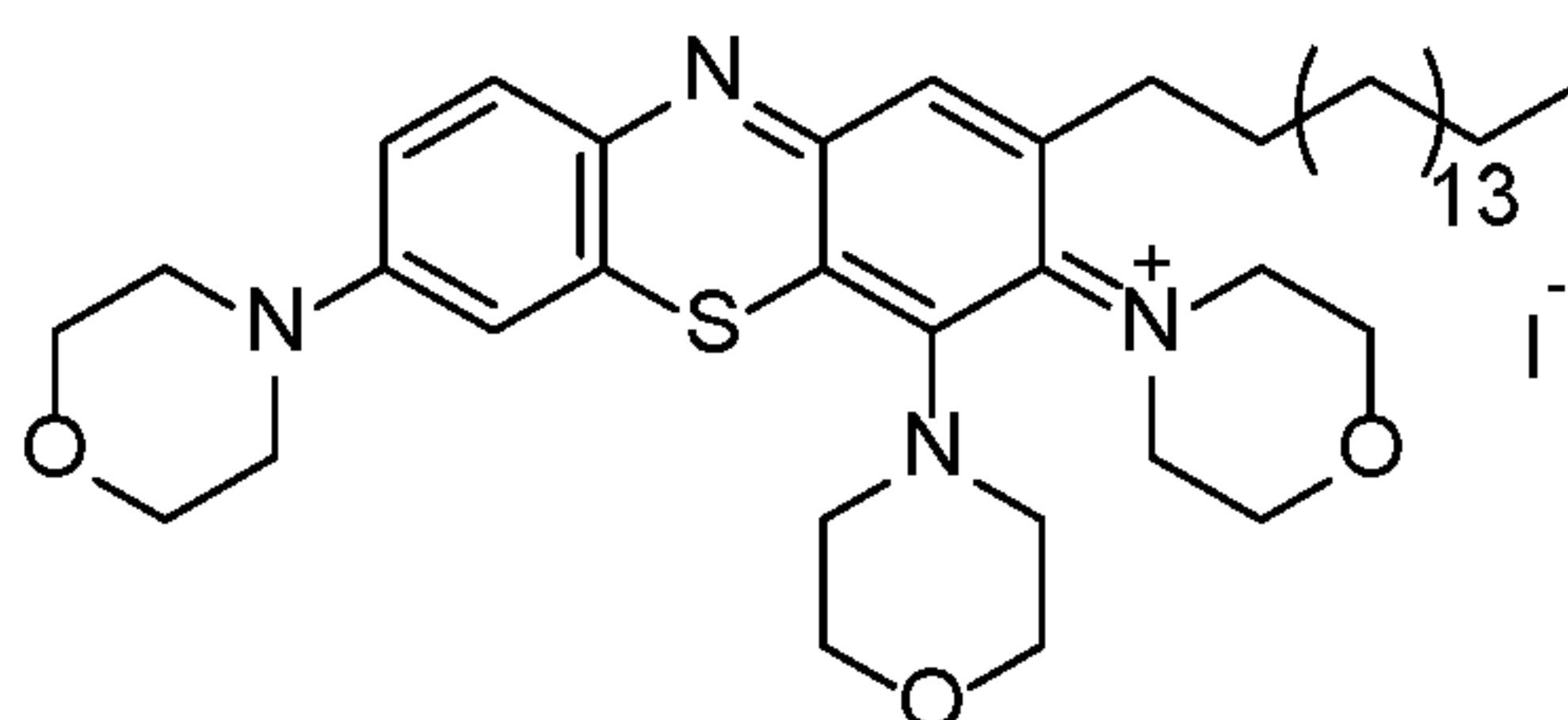
N-(4,7-bis(morpholino)-2-heptadecyl-3H-phenothiazin-3-ylidene)-N-morpholinium iodide (12)
