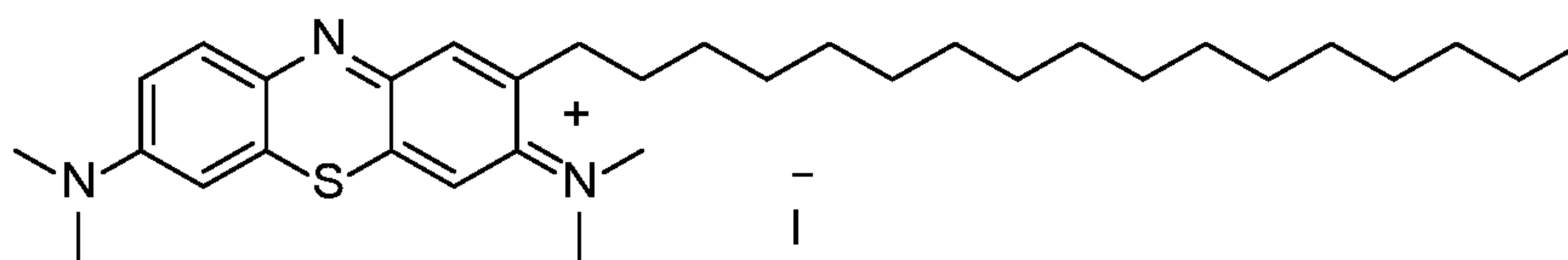
N -(7-(dimethylamino)-2-heptadecyl-3 H -phenothiazin-3-ylidene)- N -methylmethanaminium iodide (5)
