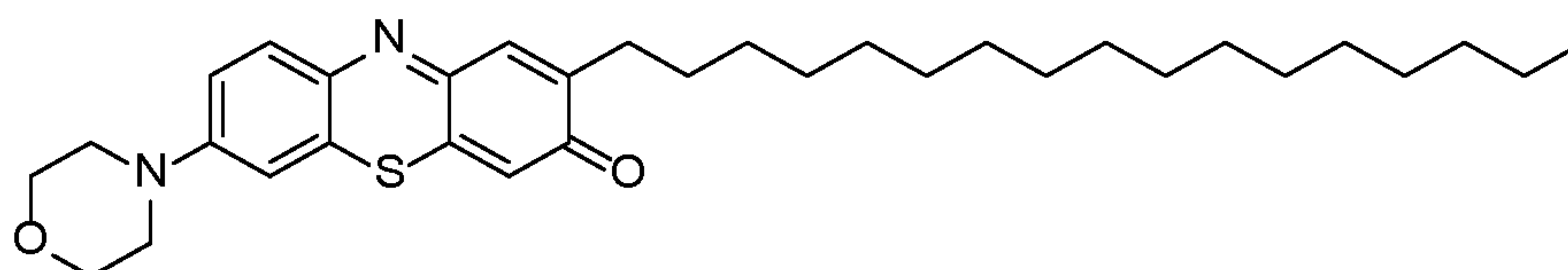
2-heptadecyl-7-(morpholine-1-yl)-3H-phenothiazin-3-one (11)
