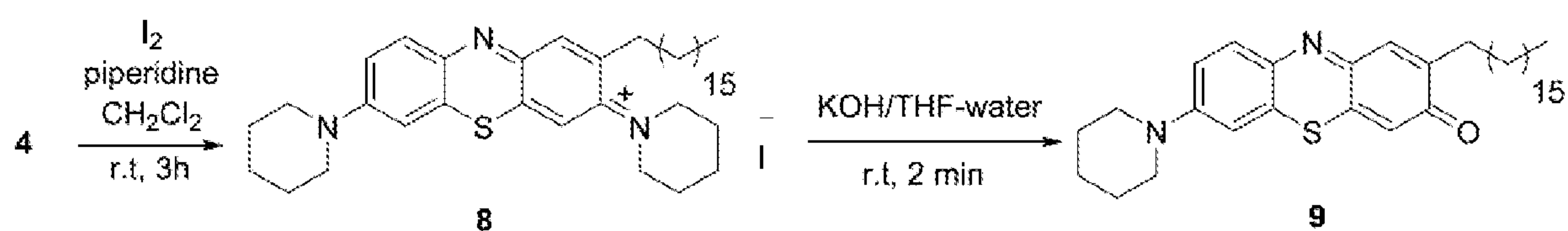
Scheme 3
