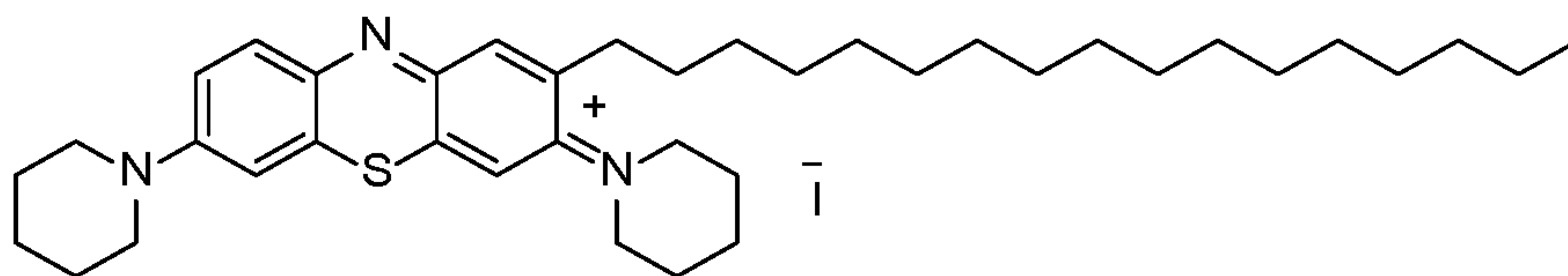
1-(2-heptadecyl-7-(piperidin-1-yl)-3H-phenothiazin-3-ylidene)piperidin-1-ium iodide (8)
