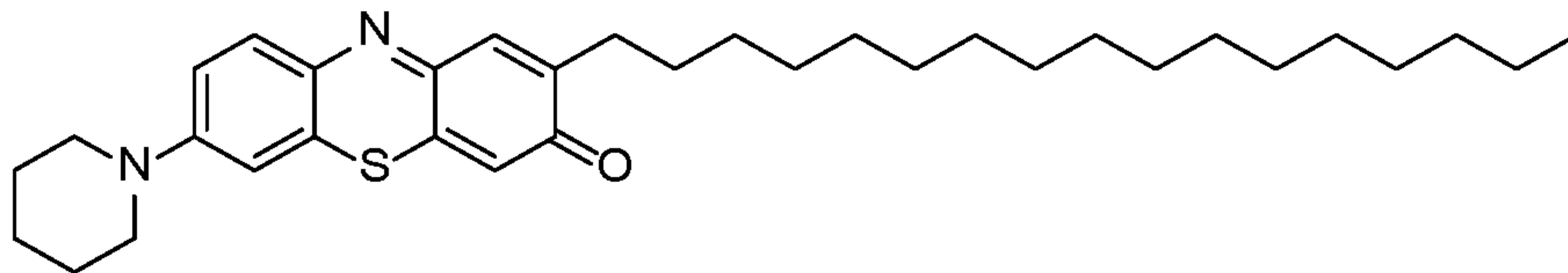
2-heptadecyl-7-(piperidine-1-yl)-3H-phenothiazin-3-one (9)
