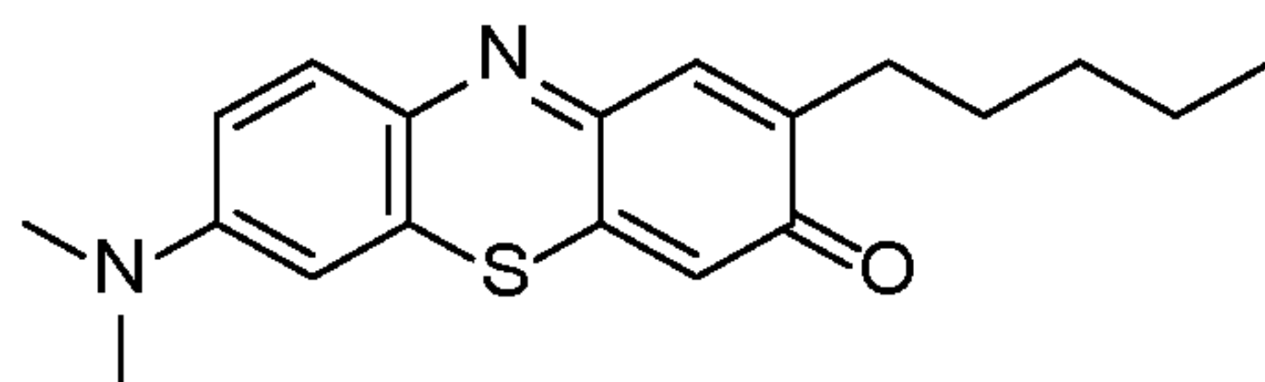
7-(dimethylamino)-2-pentyl-3H-phenothiazin-3-one (19)
