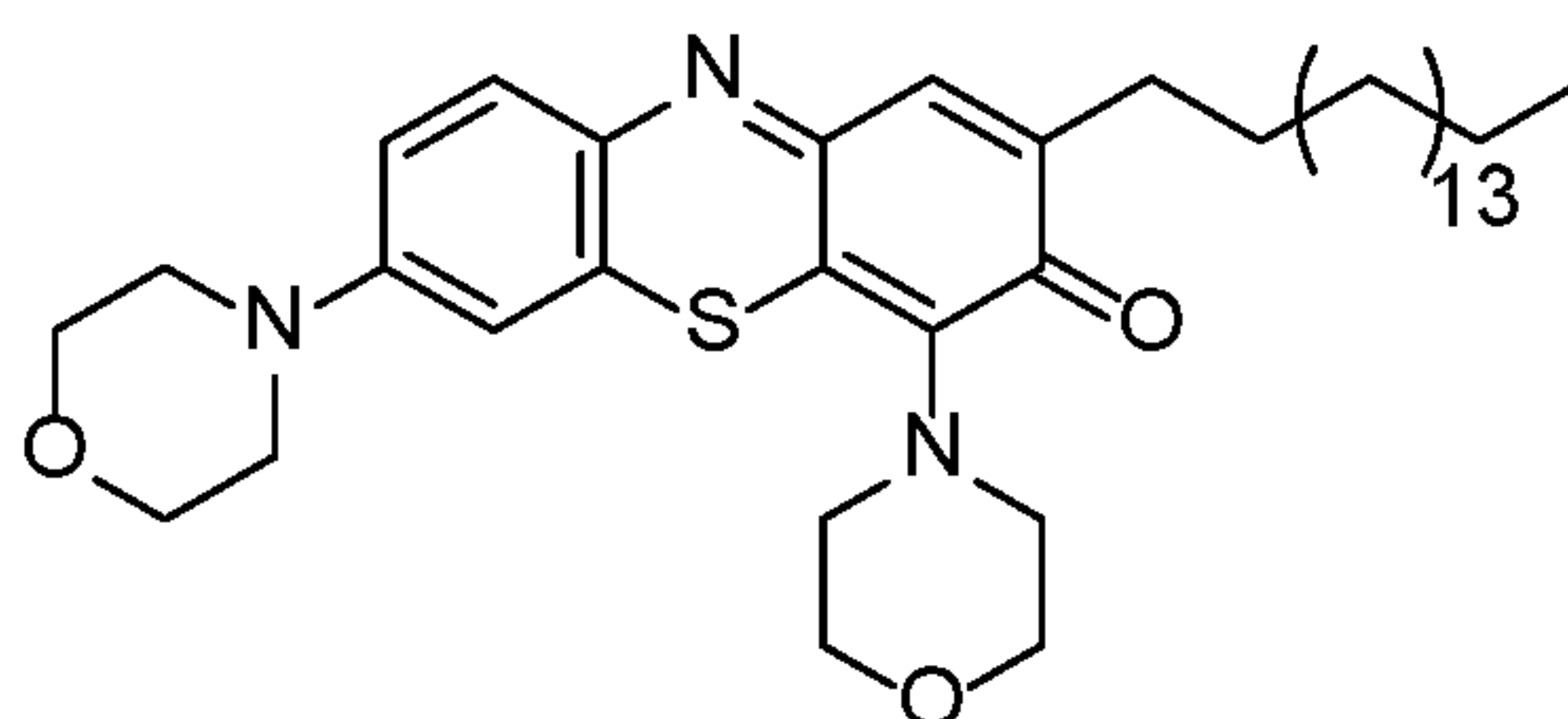
4,7-bis(morpholino)-2-heptadecyl-3H-phenothiazin-3-one (13)
