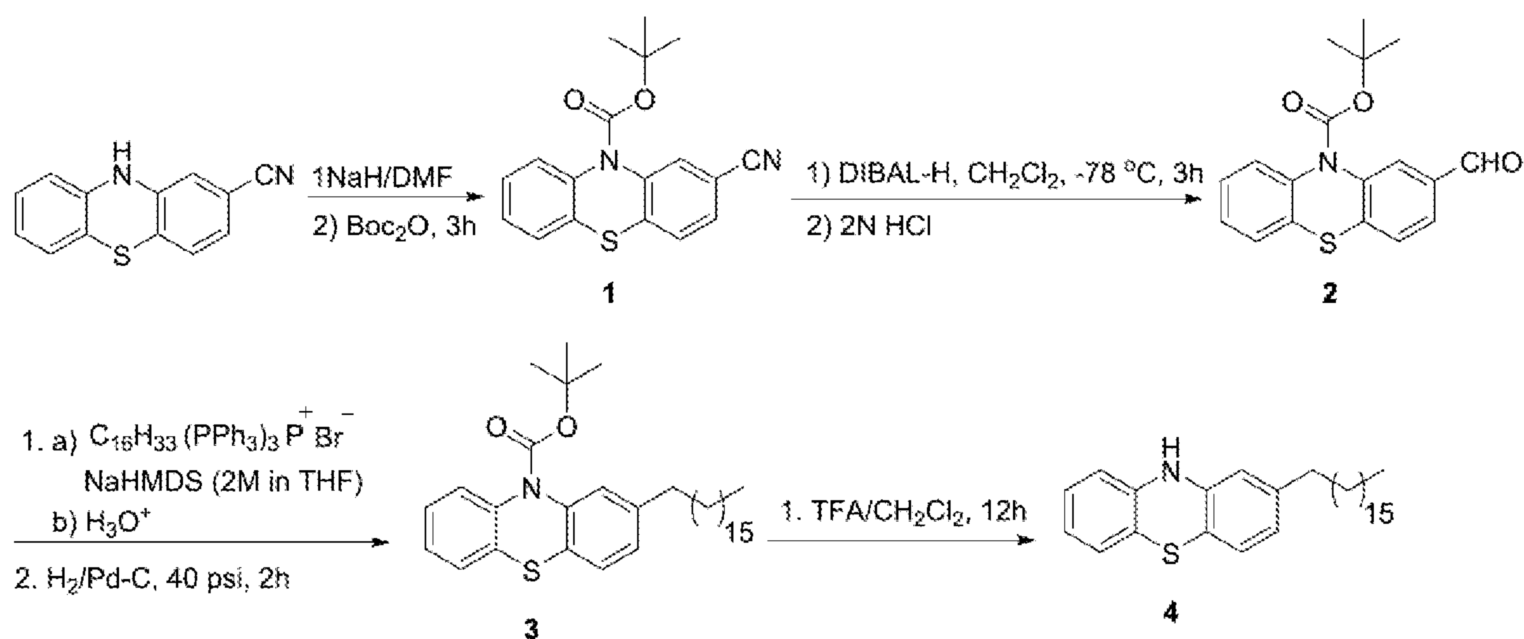
Scheme 1
