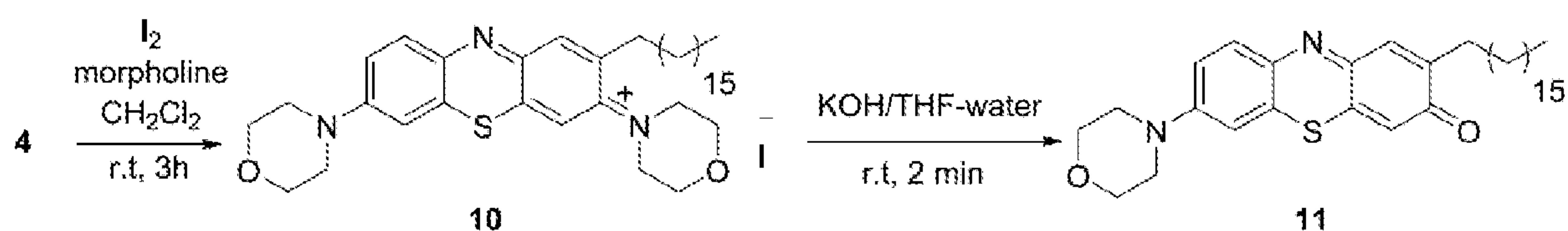
Scheme 4
