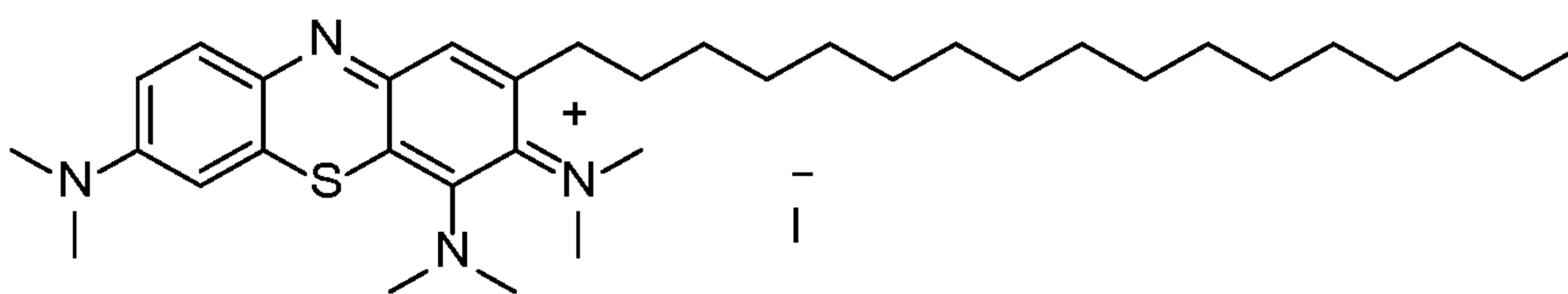
N -(4,7-bis(dimethylamino)-2-heptadecyl-3 H -phenothiazin-3-ylidene)- N -methylmethanaminium iodide (6)
