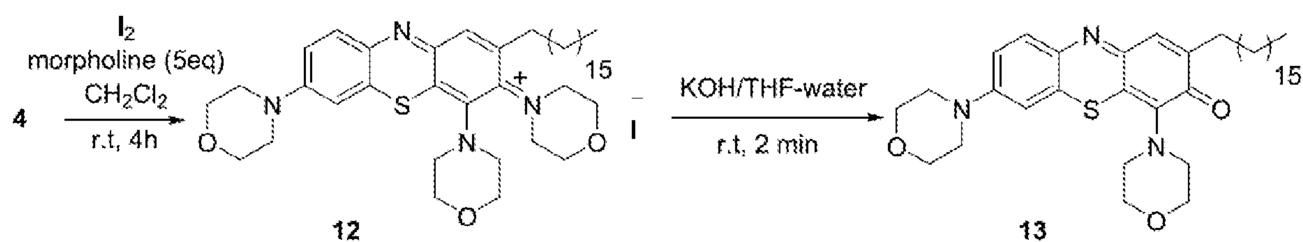
Scheme 5
