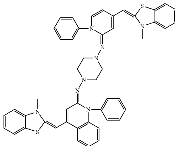
(Compound 25)
