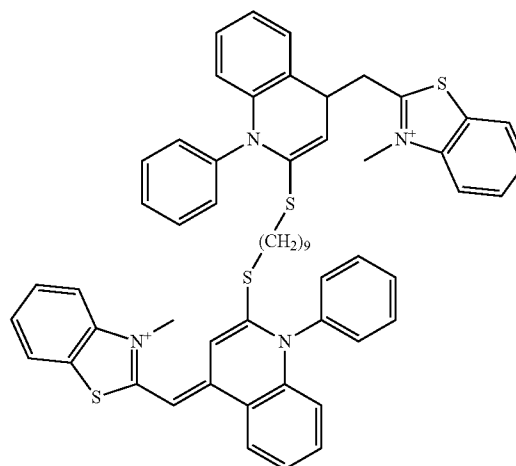
Compound 1
