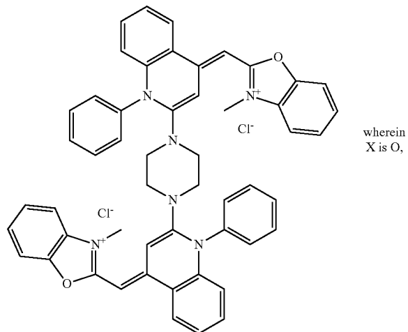
(Compound 11)
