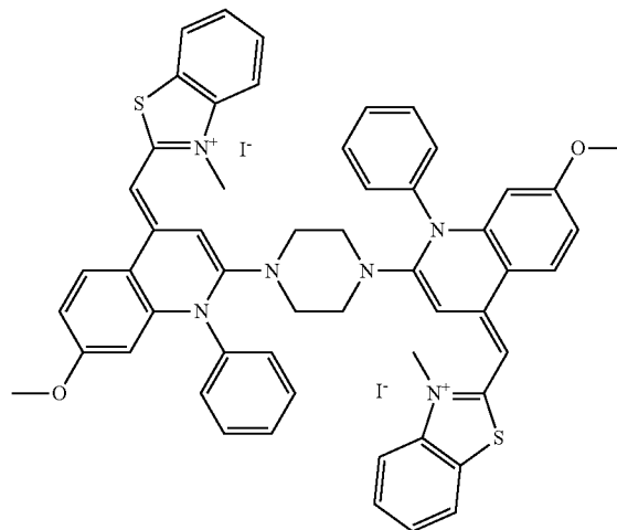
Compound 19
