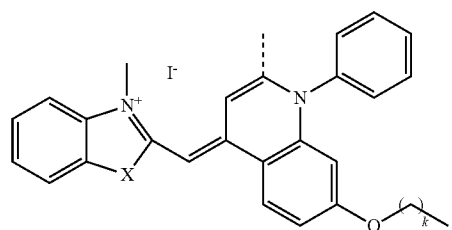
Formula (III)(e)
