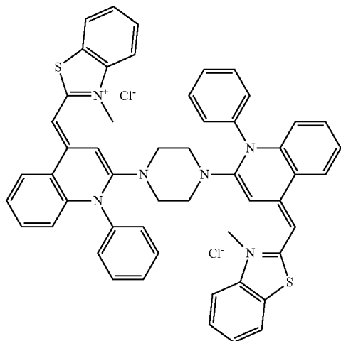
Compound 6
