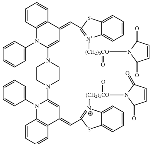
Compound 32
