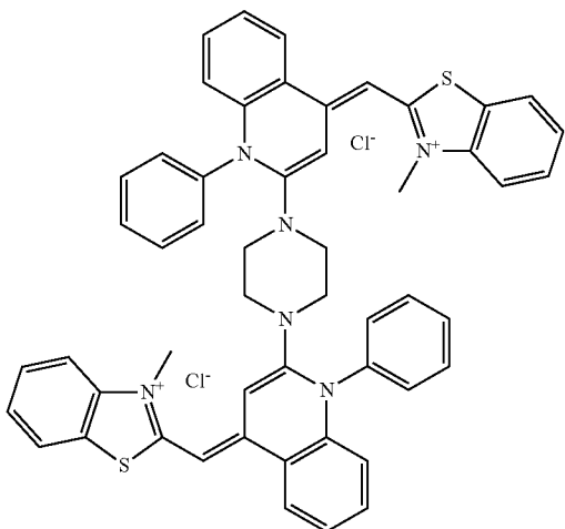
Compound 6
