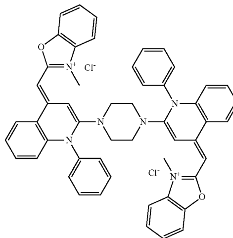
Compound 20
