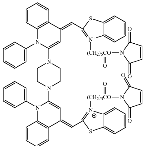
(Compound 33)
