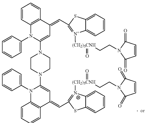
(Compound 34)
