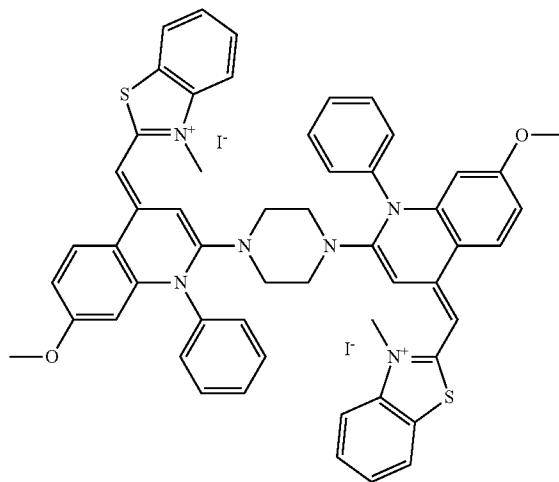
(Compound 19)
