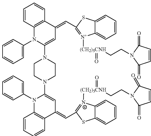
Compound 33
