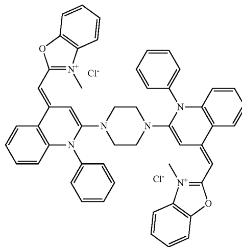
(Compound 23)
