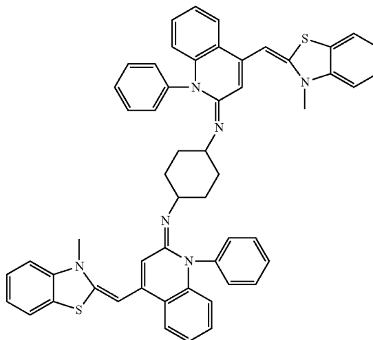
Compound 8
