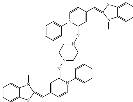
(Compound 11)
