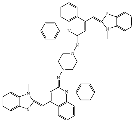
(Compound 9)
