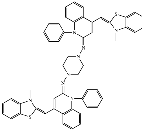
Compound 9
