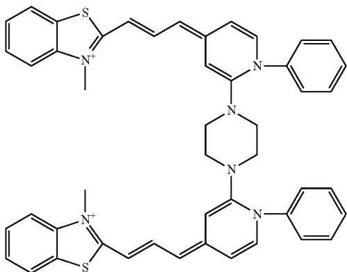
(Compound 18)
