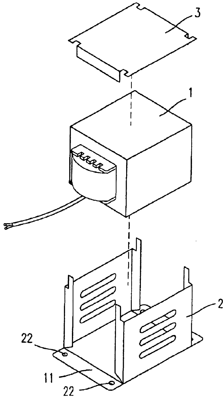
Fig. 1 (PRIOR ART)
