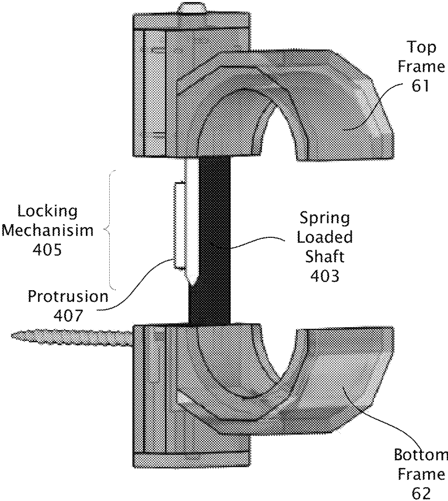
Second Example of a Locking Gun Mount 401
