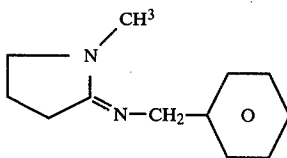
2-butyrimine-1-methyl-butyrolactam
