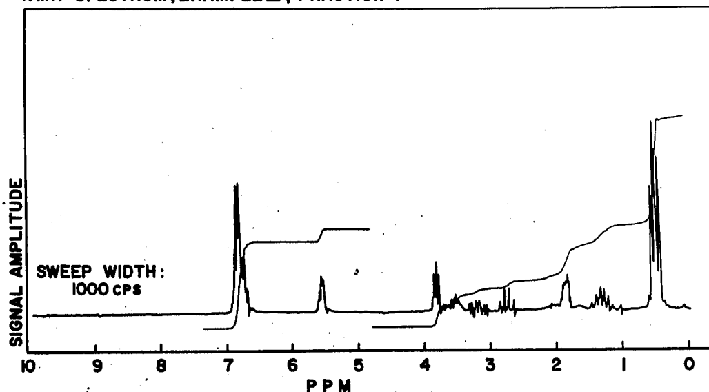
NMR SPECTRUM, EXAMPLE I, FRACTION 7
