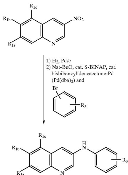
Scheme IV
