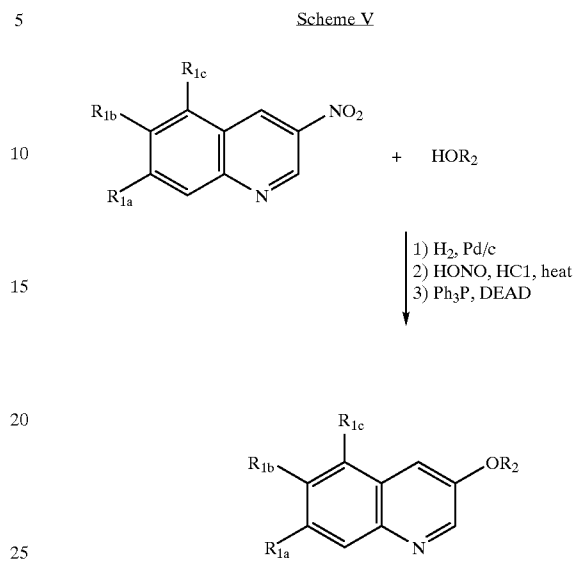
Scheme V
