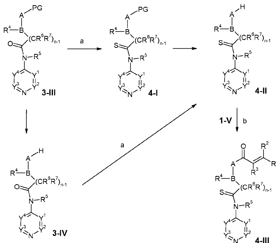
[425] Scheme 4:
