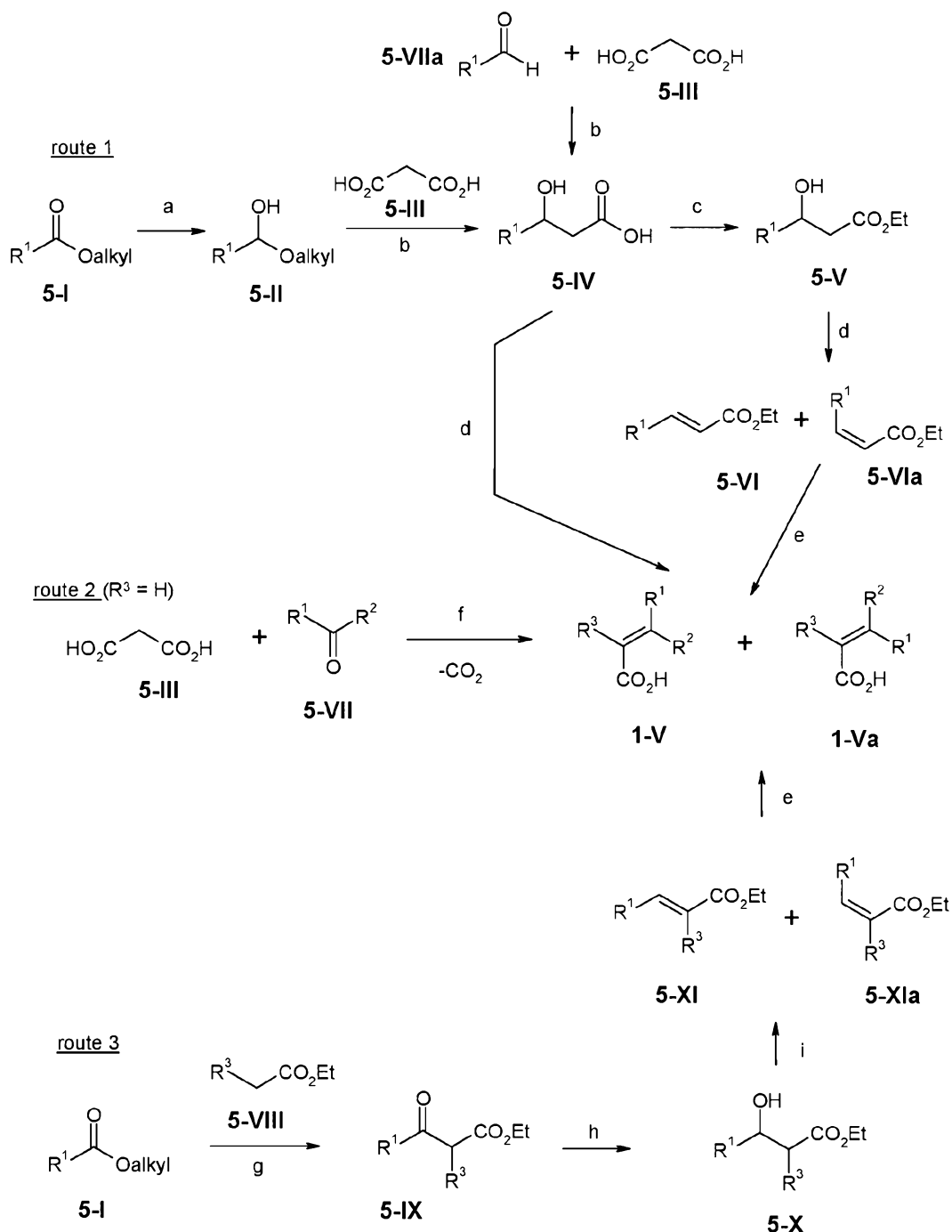
[429] Scheme 5:
