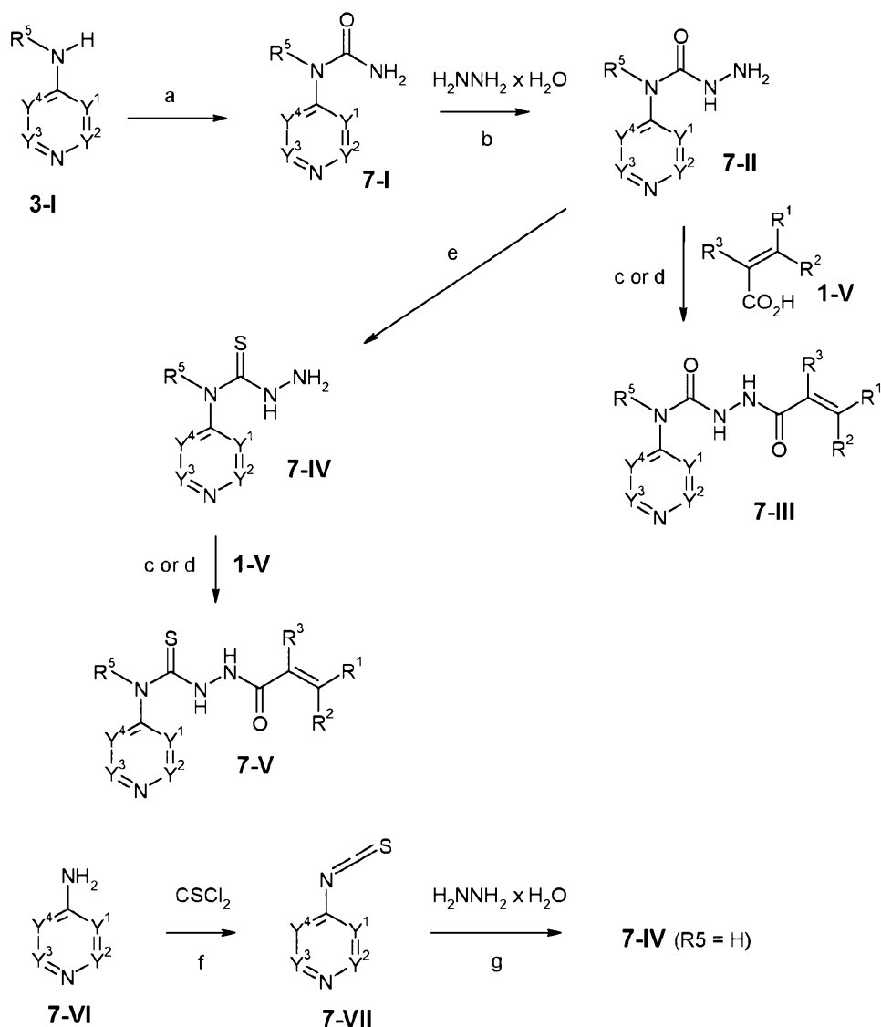
[435] Scheme 7:
