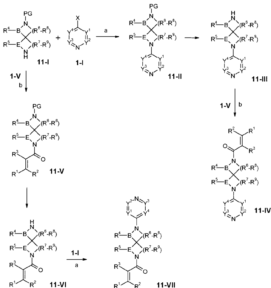
[449] Scheme 11:
