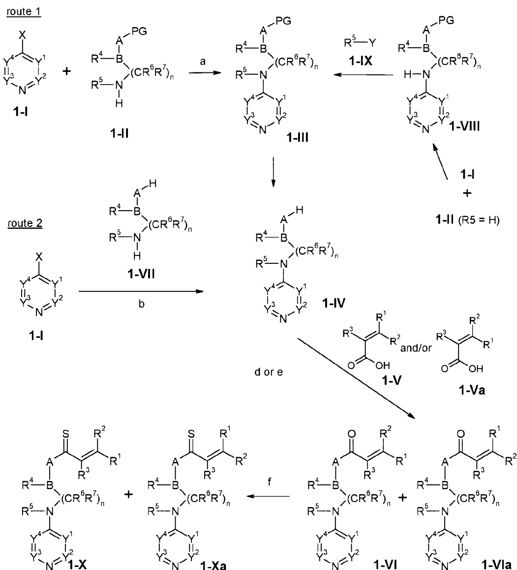
[415] Scheme 1:
