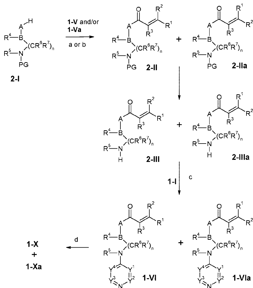
[418] Scheme 2:
