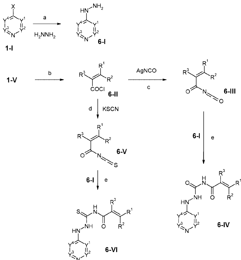
[432] Scheme 6:
