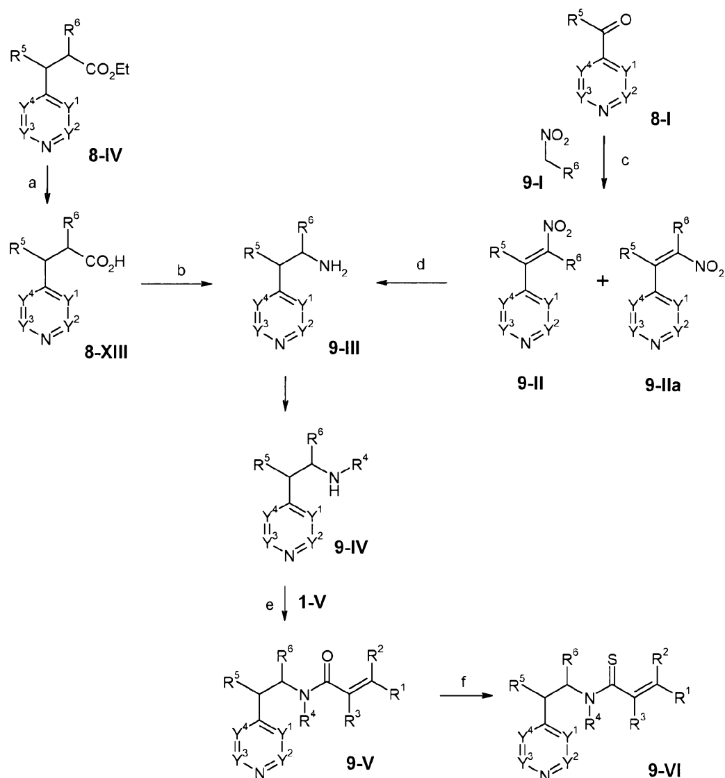
[442] Scheme 9:
