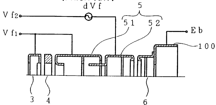
FIG. 82B (PRIOR ART)
