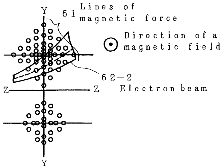
Direction of an electron beam travel
