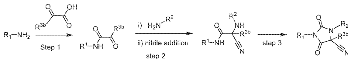
Scheme 7
