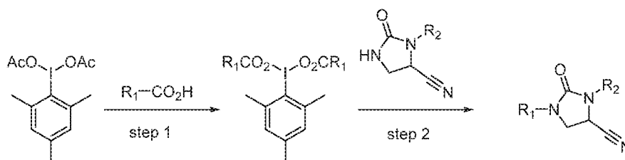
Scheme 8
