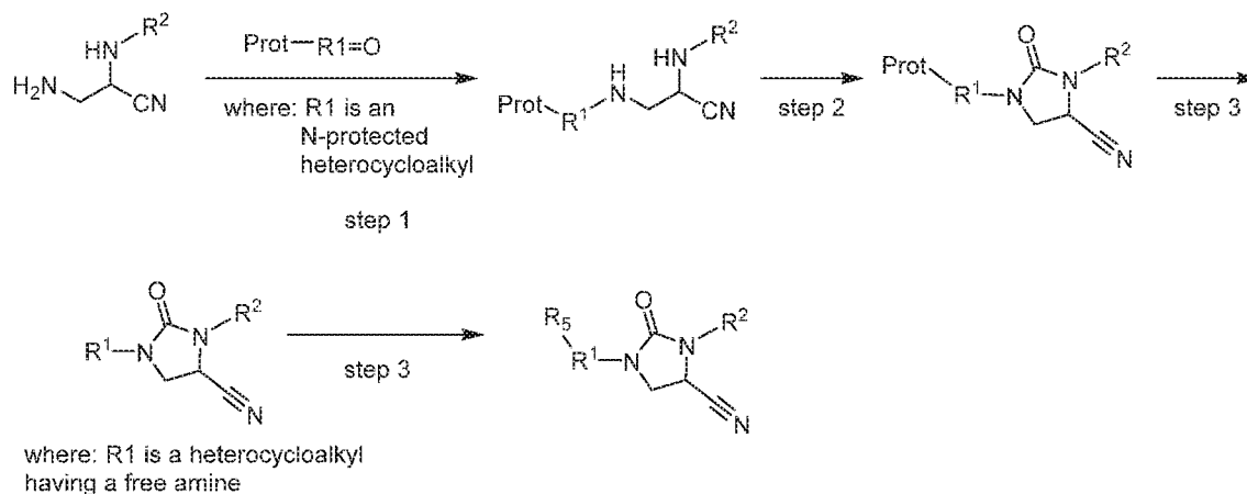
Scheme 5
