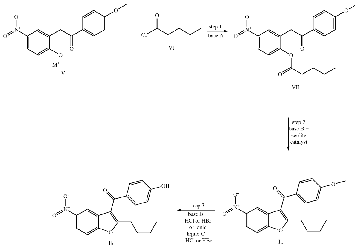
Scheme 5
