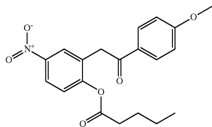
Scheme 3
