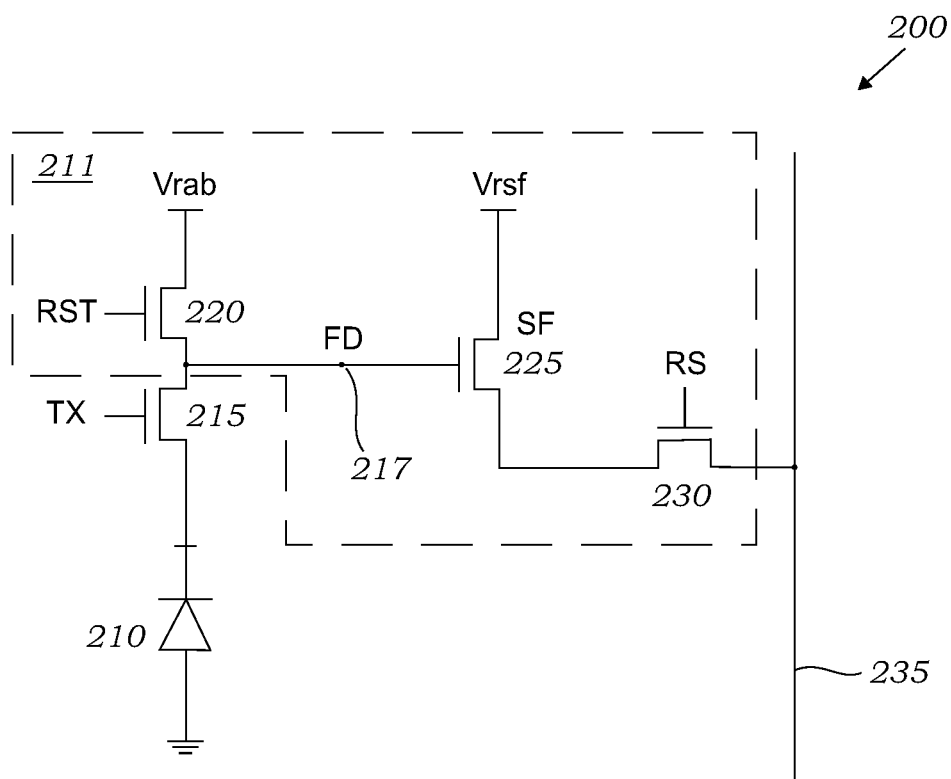
Fig. 2 (Prior Art)
