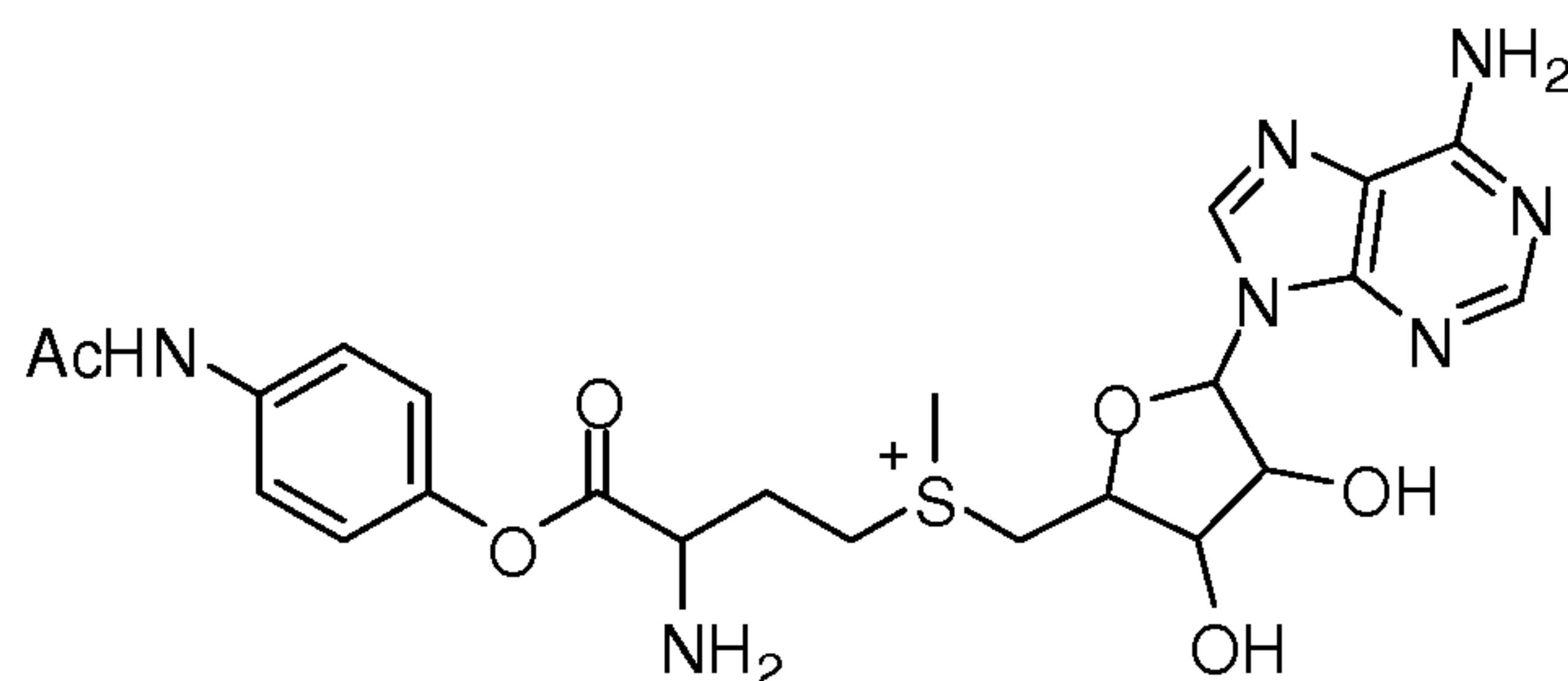
(II-I): (4-(4-acetamidophenoxy)-3-amino-4-oxobutyl)((5-(6-amino-9H-purin-9-yl)-3,4-dihydroxytetrahydrofuran-2-yl)methyl)(methyl)sulfonium;
