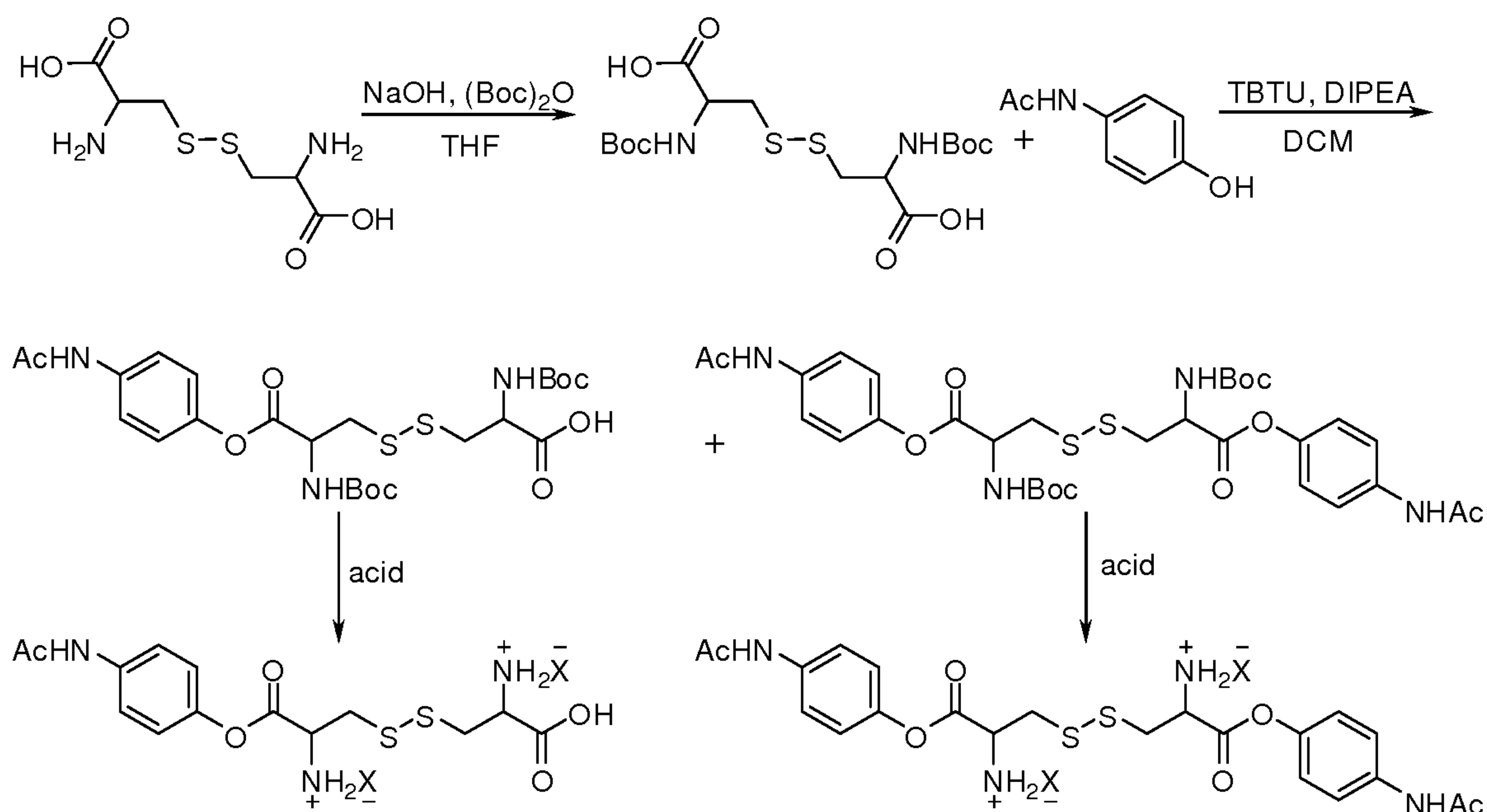
Scheme III.
