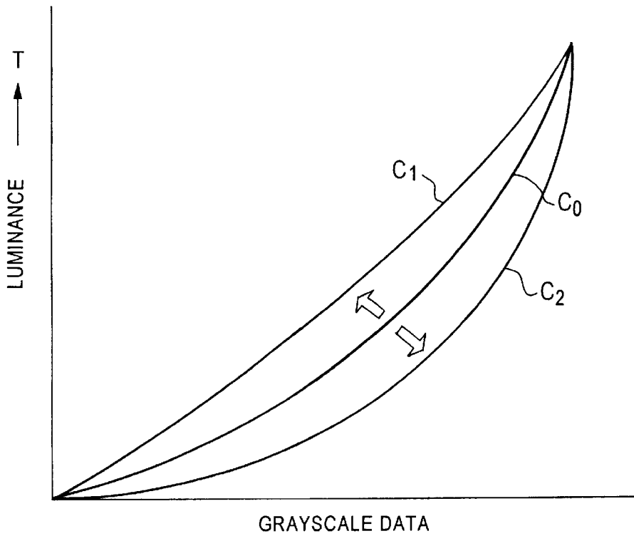
Fig. 19 (PRIOR ART)
