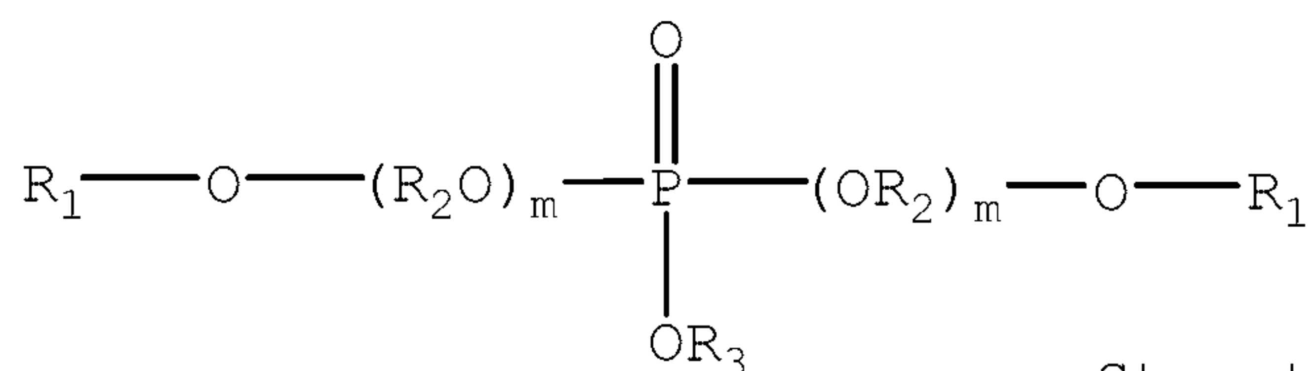
Structure (XIb)
