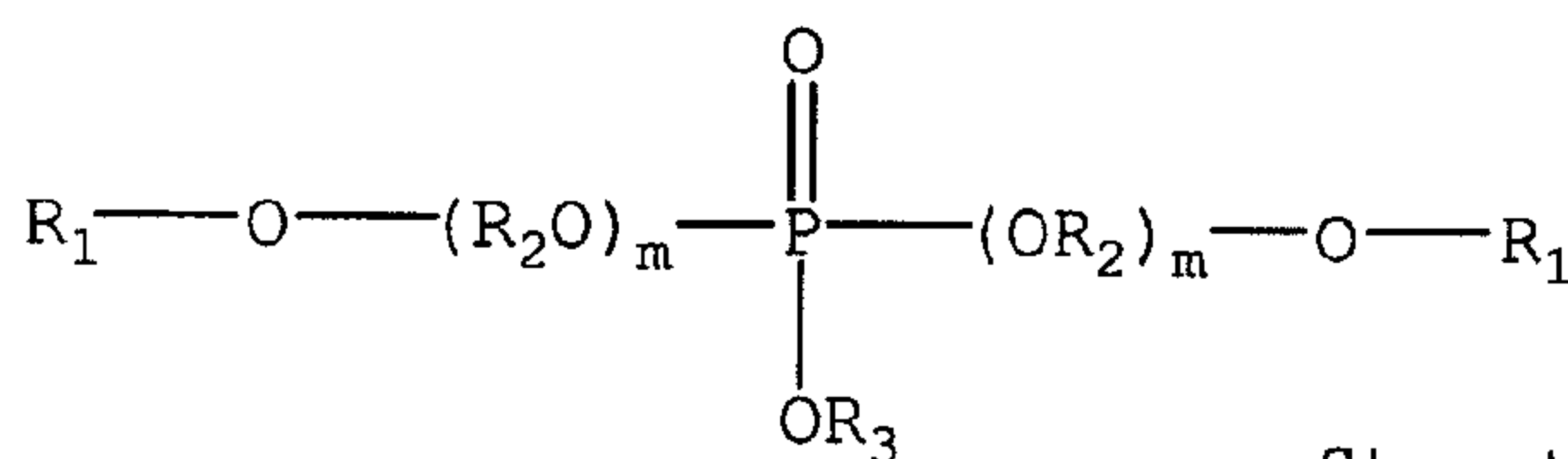
Structure (XIb)
