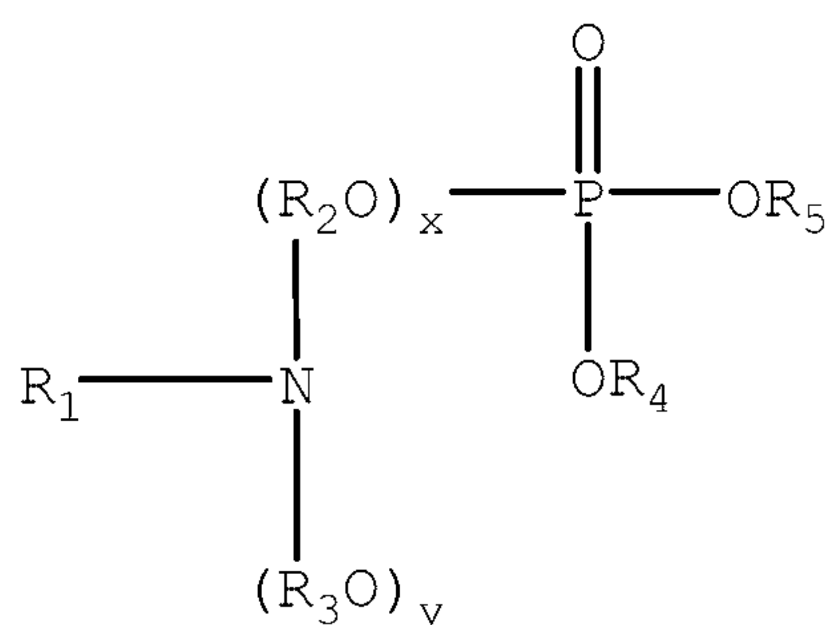
Structure (IXa)
