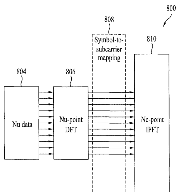
Localized DFT-s-OFDMA
