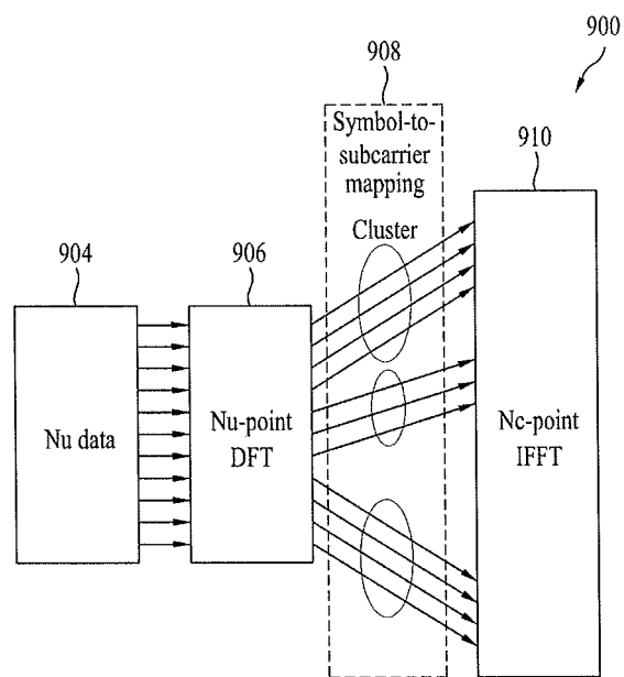
Clusters DFT-s-OFDMA
